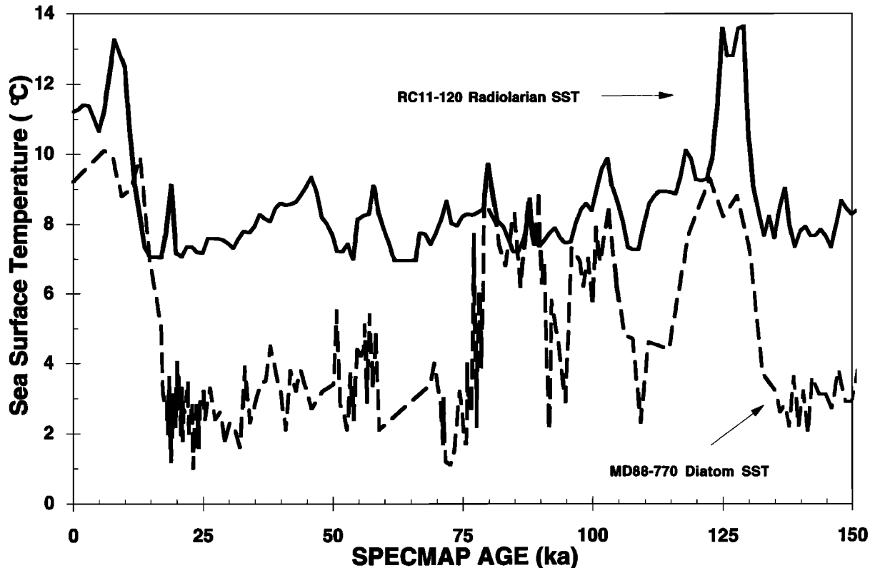
Fig. 7. Sea surface temperature (SST) records from RC11-120 (44°S, 80°E) (solid line) and MD88-770 (46°S, 96°E) (dashed line) both plotted on the SPECMAP timescale. The RC11-120 record is from Hays et al. [1976a] based on a radiolarian transfer function. The SST record from MD88-770 is based on a diatom transfer function [Pichon et al., 1992]. The two records show similar glacial to interglacial temperature shifts of 6°-8°C. The SST record from RC11-120 is systematically higher than that of MD88-770. One explanation for this systematic difference is that the radiolarian transfer function is not reliable at temperatures below 7°C.
