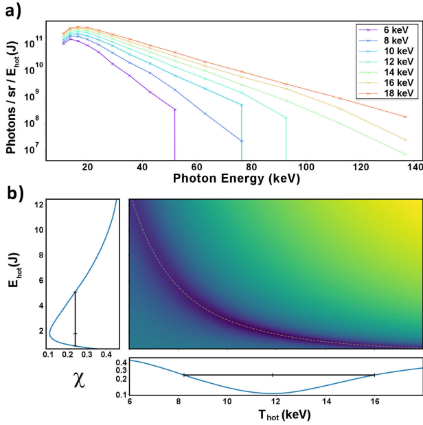
FIG. 6. a) Synthetic Bremsstrahlung X-ray emission spectra obtained by HE populations of different T_{hot} temperatures, resulting from Geant4 simulations. b) Typical heat map of \chi^2 for different (T_{hot}, E_{hot}) combinations; the gray line represents the locus of minimum chi squared, while the projections on the axes show that the optimal fit consists of T_{hot} = 12 keV and E_{hot} = 2 J.
