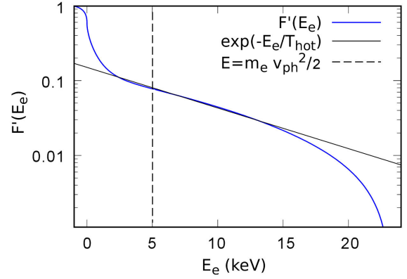
FIG. 10. Complementary distribution function F'(E_e) as a function (blue line) of the electron energy E_e from a typical simulation with SIERA for a RPP beam at I_0 = 10^{16} W/cm 2 and for a density ramp 0.02 < n/n_c < 0.10 . The tail of the distribution evolves versus a HE distribution (black line) \sim \exp(-E_e/T_{hot}) with T_{hot} = 8 keV here, i.e. in the range of the experimentally observed values. The position of the energy corresponding to the EPW phase velocity is indicated (dotted line at \sim 5 keV).
