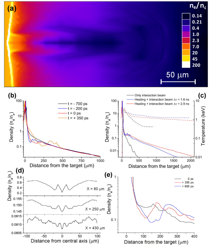
FIG. 2. Density and temperature profiles obtained from hydrodynamic simulations carried out with the DUED code. (a) 2D map of electron density in the high density region taken at the peak of the interaction pulse, in case of delay time \Delta\tau = 2.9 ns; (b) longitudinal profiles of electron density at different times of interaction in case of delay time \Delta\tau = 2.9 ns; (c) longitudinal profiles of electron density and temperature taken at the peak of the interaction pulse for delay times \Delta\tau = 1.6 ns (blue lines), \Delta\tau = 2.9 ns (red lines) and for the case where heating beams are not used (black lines); (d) transverse density profiles taken at different distances from the target surface in the same conditions as (a); (e) temporal evolution of the dip in the density profile.
