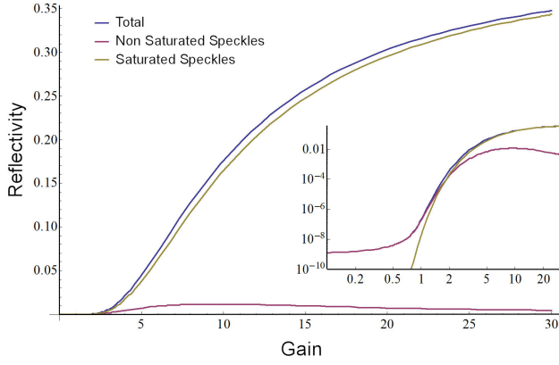
FIG. 7. Values of total SRS reflectivity (blue) calculated by using Eq.(2). Red and Yellow lines indicate the contributions given by non saturated (first term in Eq.(2)) and saturated (second term in Eq.(2)) speckles. The inset represents the graph in Logarithmic scale.
