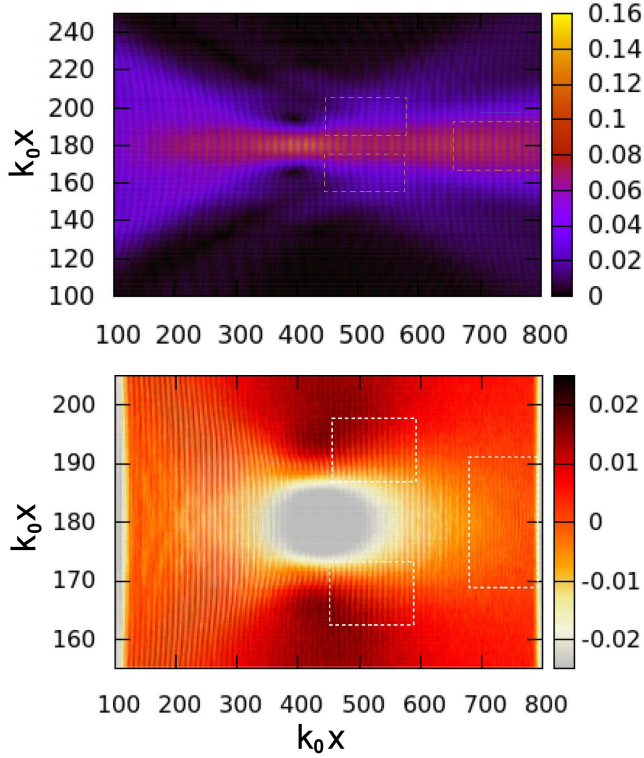
FIG. 11. Normalized transverse field strength e|E_y|/(m_e\omega_0c) (upper subplot) and electron density perturbations (lower subplot) (n_e(x,y) - n_0(x))/n_0(x) as a function of space for a single laser speckle with peak field strength e|E_y|_{in}/(m_e\omega_0c) = 0.1 . The self-focusing speckle shows an elongated structure on axis ( k_0y = 180 ) with a field strength higher than the initial value |E_y|_{in} . The laser light enters from the left, x = 0 . The dashed lines in both subplots indicate the zones where SRS is amplified: the density perturbations (note that the range shown in y is reduced with respect to the upper subplot) exhibit plasma wave oscillations in the periphery of the field hot spot, but not in the depleted zone inside. SRS-driven EPW are in particular present at the rear on axis and in side wings. SBS-driven ion acoustic wave are found in the front part (PIC simulations show generally too high values).
