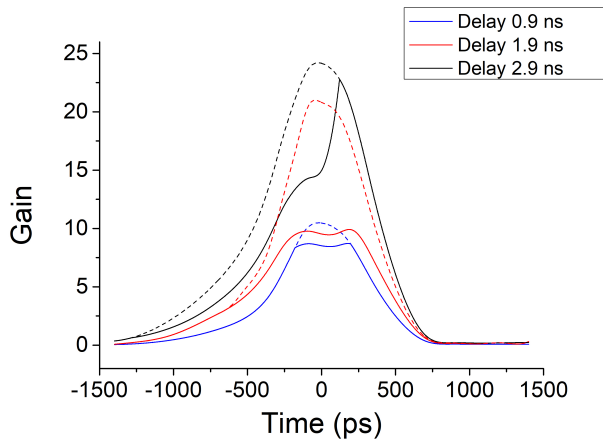
FIG. 8. Time Evolution of SRS gain calculated by using Eq.(4) for the laser beam configurations with time delay \Delta\tau = 0.9, 1.9 and 2.9 ns between heating and interaction beams. Dashed and solid lines indicate the gains calculated by using the Rosenbluth theory and the modified expression Eq.(4) accounting for Landau damping into a speckle, respectively.
