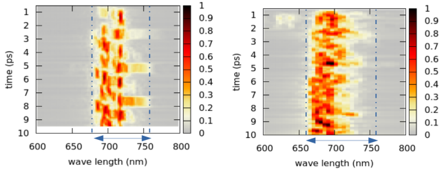
FIG. 9. Spectra of the backscattered light from simulations with SIERA for a RPP beam at I_0 = 10^{16} W/cm 2 and for a density ramp 0.02 < n/n_c < 0.10 , left/right subplots with/without taking into account kinetic effects.
