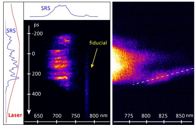
FIG. 5. Time-resolved SRS spectra acquired in two different shots by the Hamamatsu C7700 (on the left) and C5680 (on the right) streak cameras. Time resolution is 18 ps. The laser fiducial in the left image allowed to determine the absolute timing of the interaction laser peak. Left and right panels show the SRS spectra scattered at low and high plasma densities, respectively. The dashed line shows the spectral shift of SRS scattered light with time at densities around 0.1 n_c .
