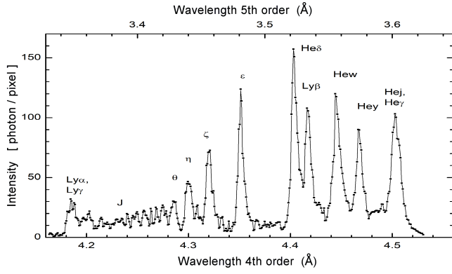
FIG. 3. X-ray spectrum of K-shell Chlorine emission from H- and He-like atoms. The measured spectrum includes the contributions of the 4 th and of the 5 th diffraction order of the crystal.
