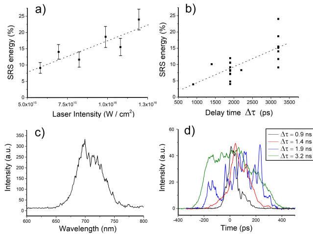
FIG. 4. Experimental results. a) SRS reflectivity versus laser intensity for a set of selected data with fixed values of \Delta\tau = 3.2 ns and \Delta x_{foc} = -150 \mu\text{m} ; b) SRS reflectivity versus the delay time \Delta\tau between heating and interaction beams; c) Typical SRS spectrum. d) Time profile of SRS light in shots with different delay time \Delta\tau . In subplot a) error bars of 20% have also been reported for reference.
