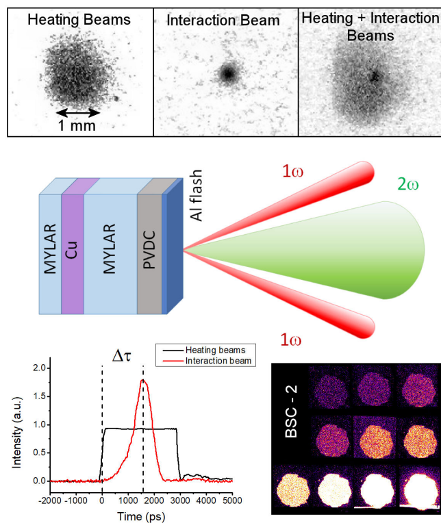
FIG. 1. Top, pinhole camera images of hard X-ray emission from plasmas induced by the heating pulses, by the interaction pulse and by all the beams. Middle, sketch of the beam configuration in the vertical plane and target structure. Bottom-left, timing of the laser beams (relative intensity is arbitrary). Bottom-right, image plates signal, obtained in calibration shot on a copper targets, acquired by the Bremsstrahlung Cannon looking at the rear side of the target; the intensity is proportional to PhotoStimulated Luminescence (PSL).
