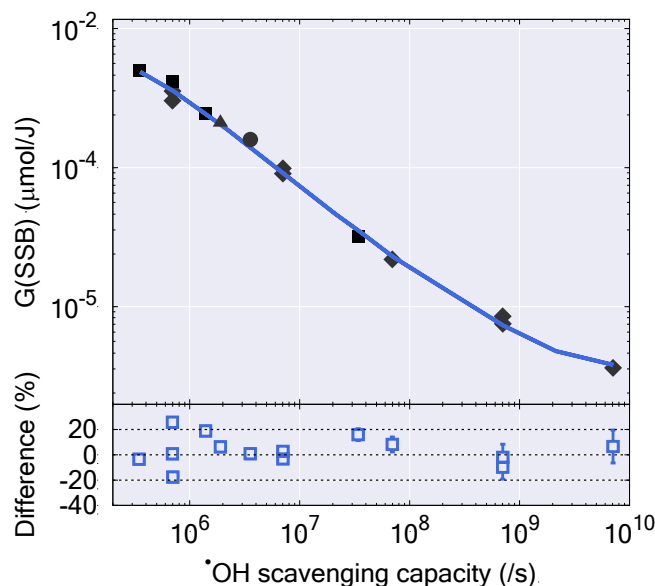
Figure 3 Total calculated SSB yields (direct plus indirect) as a function of \bullet\text{OH} scavenging capacity (solid lines). Measured data for pUC18 is from \blacksquare (Milligan et al 1993), \blacklozenge (Milligan and Ward 1994), and \bullet (Milligan et al 1996). Measured data for pUC19 \blacktriangle is from (Perry et al 2021). Percentage differences ( \square ) between calculated to measured data are shown in the bottom figure. The dotted lines are margins from experimental uncertainty. Error bars are displayed when bigger than the symbol, represent statistical uncertainties from Monte Carlo simulations, one standard deviation.
