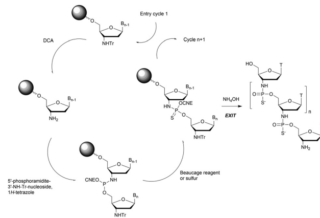
Scheme 30 Synthesis cycle of NPS-ODN.
