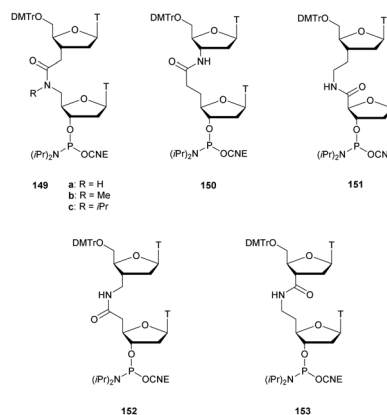
Fig. 20 Chemical structures of the AM-dithymidine phosphoramidite building blocks 149–153 synthesised by Just 384 and De Mesmaeker. 385,386
