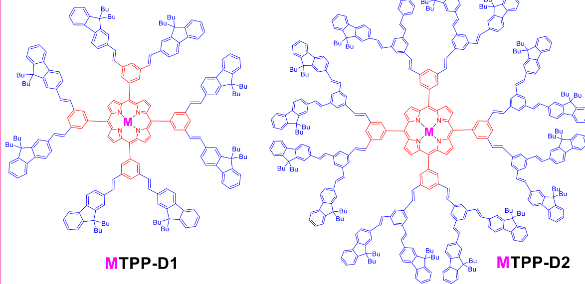
Figure 1 a) Reference compounds; b) Previously reported alkynyl-bridged free-base porphyrin dendrimers ( T series ) based on TPP ( TPP-T1 and TPP-T2 ); c) New porphyrin dendrimers ( D series ) based on TPP ( MTTP-D1 and MTTP-D2 ; M = 2H, Zn).
