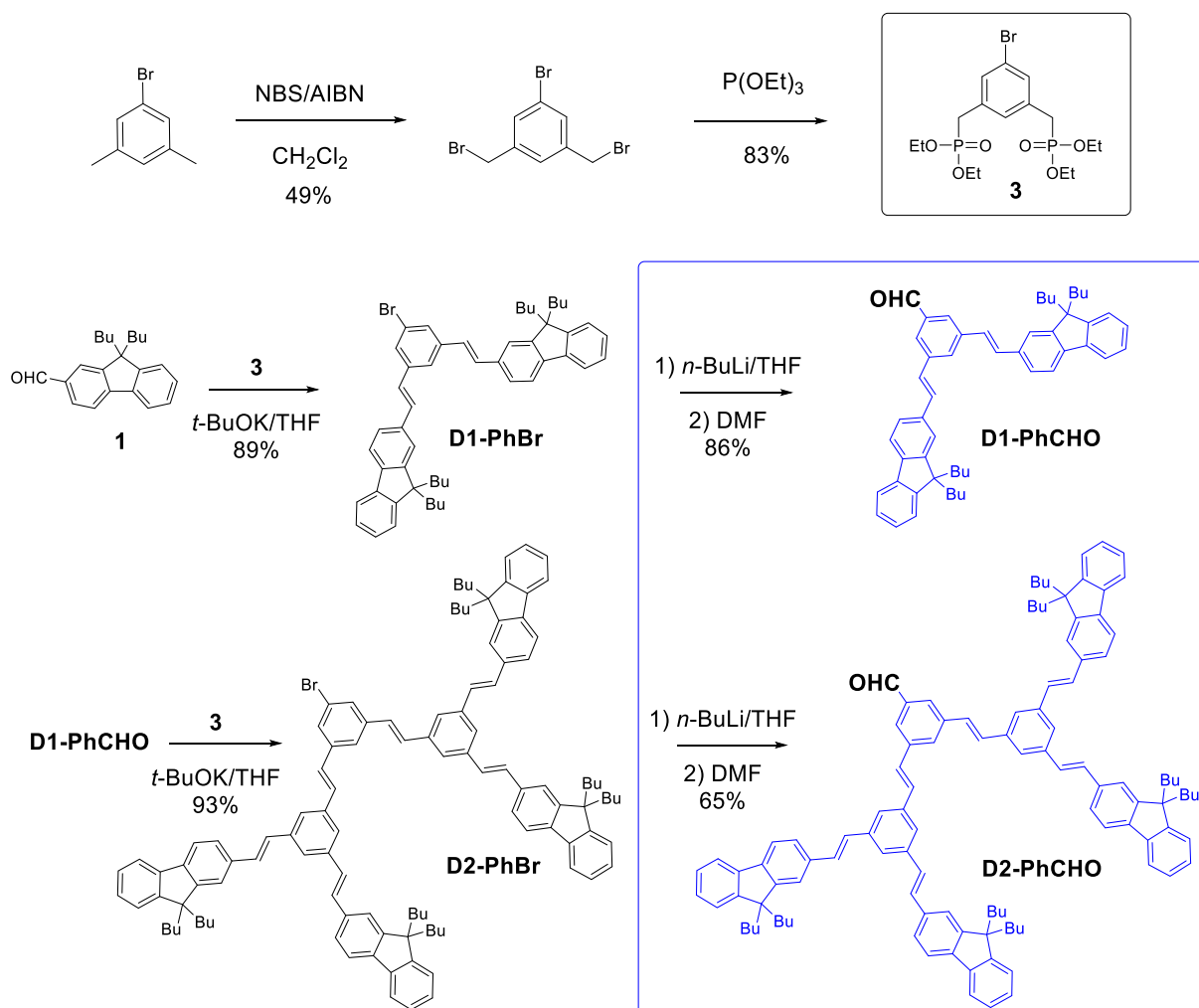
Scheme 1. Synthetic routes for alkene-bridged dendrons D1-PhCHO 13 and D2-PhCHO .
