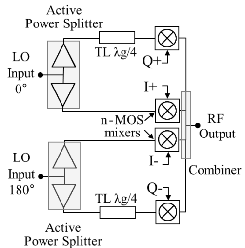
FIGURE 1. Synoptic of the overall MMIC topology (modulation configuration).
