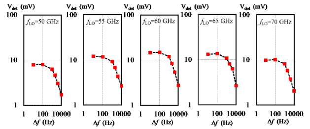
FIGURE 9. Measured video bandwidth vs. RF frequency: voltage detected as a function of frequency difference f_{RF} - f_{LO} .
