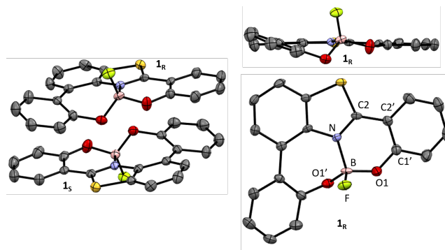
Figure 2. X-ray crystal structure of 1 with thermal ellipsoids at 50% probability: asymmetric unit (left) with 1 R and 1 S ; in-plane (top right) and top-face (bottom right) views of 1 R . Boron in pink, carbon in grey, nitrogen in blue, oxygen in red, fluorine in green and sulfur in yellow; H atoms omitted for clarity.
