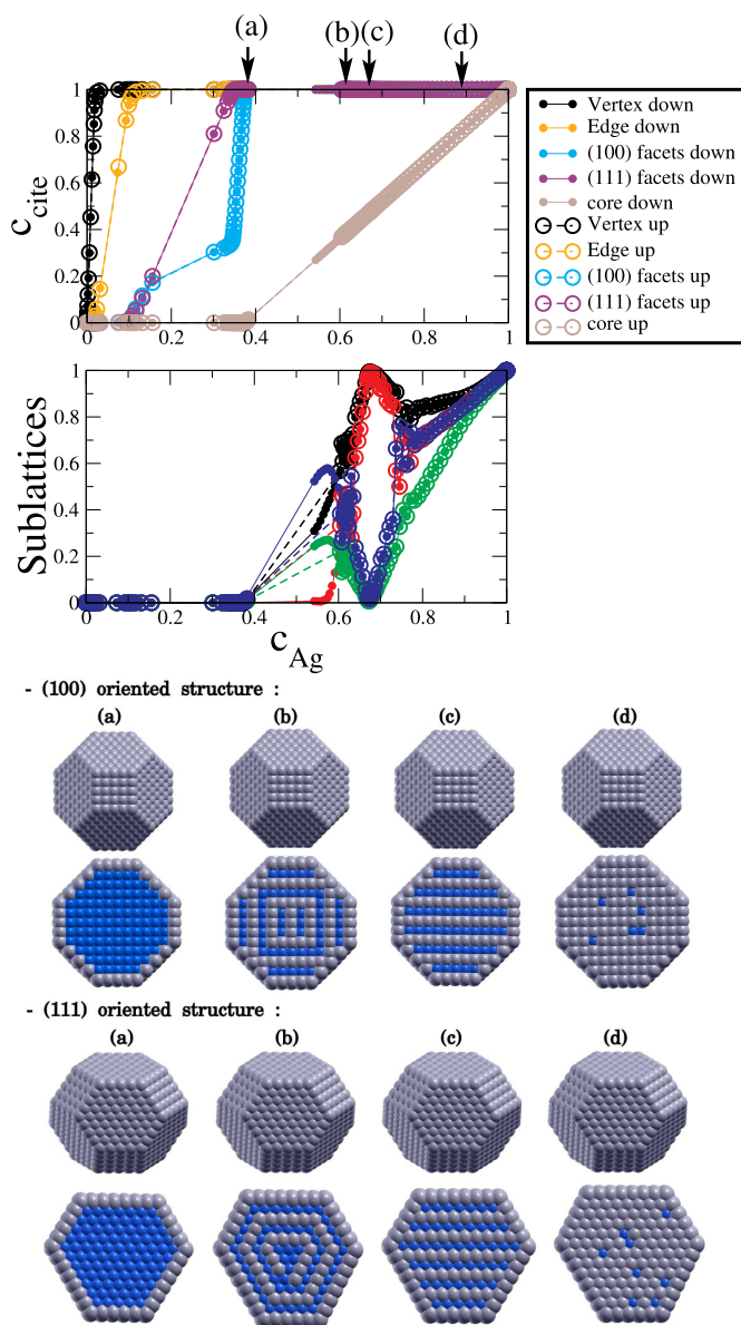
Fig. 12. Segregation isotherms of TOH_{1289} cluster at 500 K with the same legends as in Fig. 11 and the associated structures.
