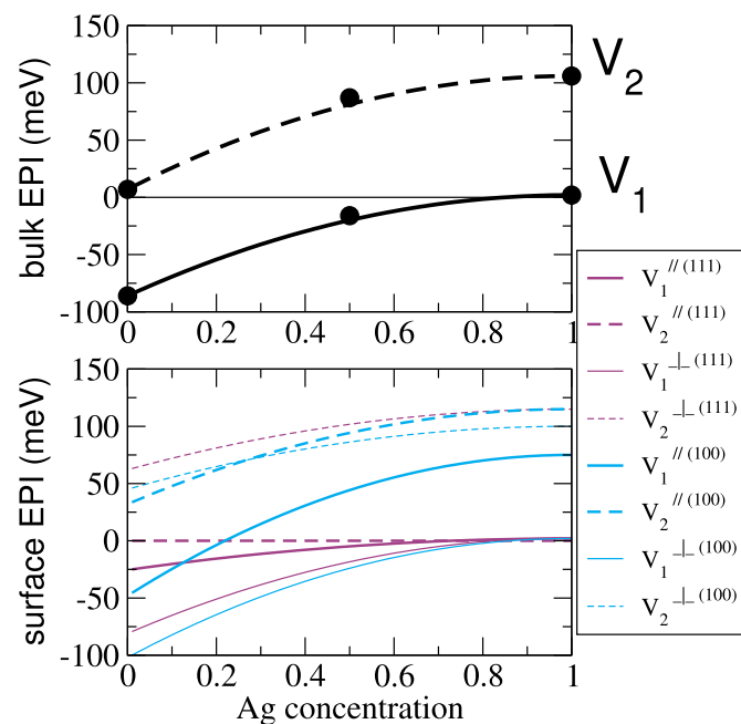
Fig. 2. Effective pair interactions (EPIs) at first and second neighbors as a function of the silver concentration in bulk (top graph) and at (111) and (100) surfaces (bottom graph).
