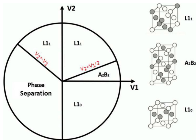
Fig. 1. Ground state diagram of an Ising model for Effective Pair Interactions (EPIs) on fcc lattice at first and second neighbors [12,23,27].
