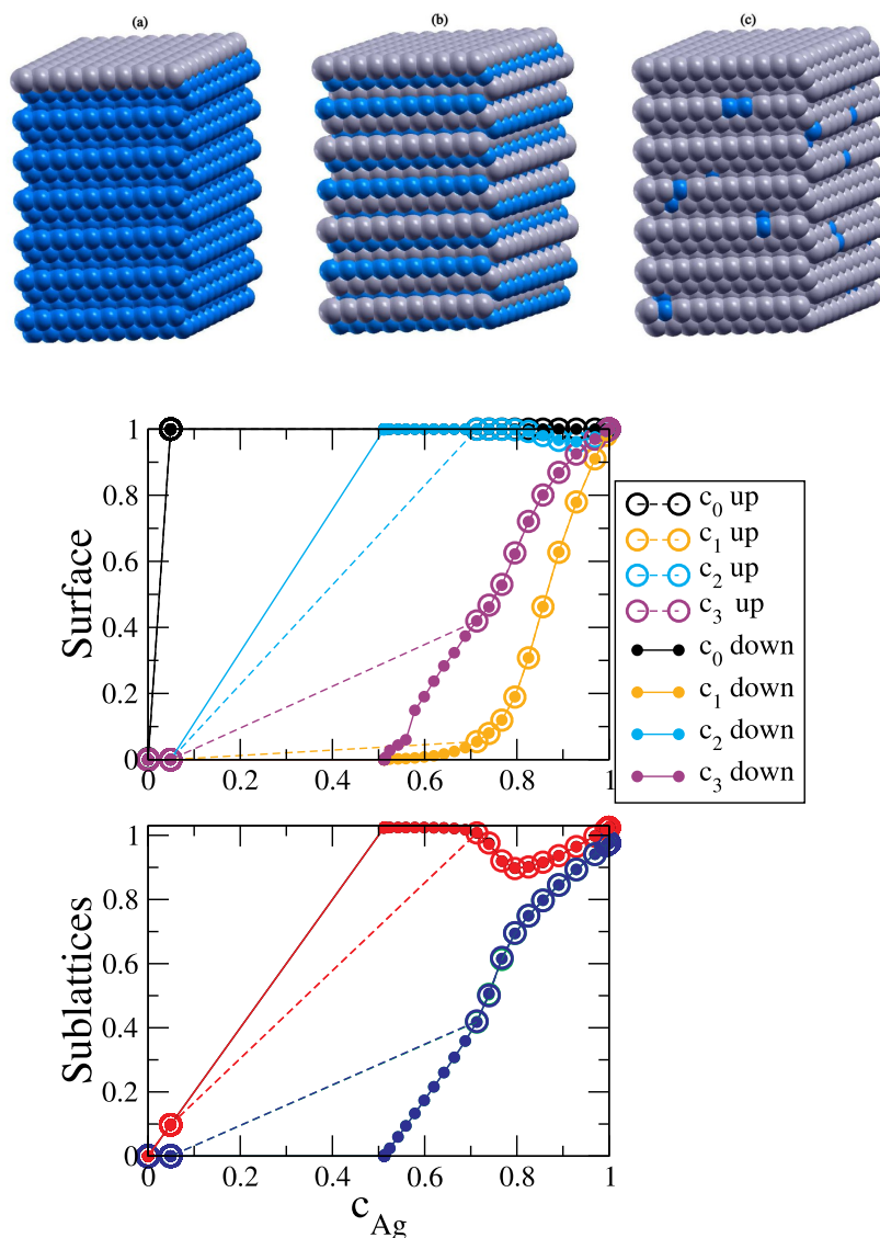
Fig. 9. Segregation isotherms of the (111) surface at 300 K. The slabs are illustrated on top for three characteristic concentrations (a) below 5%, (b) 50% and (c) above 80% with Ag atoms in grey and Pt atoms in blue. Then the first four layers concentrations starting from the surface c_0 , c_1 , c_2 and c_3 are plotted in the top graph and finally the core sublattices concentrations are plotted in the bottom graph as a function of the global Ag concentration. (For interpretation of the references to color in this figure legend, the reader is referred to the web version of this article.)
