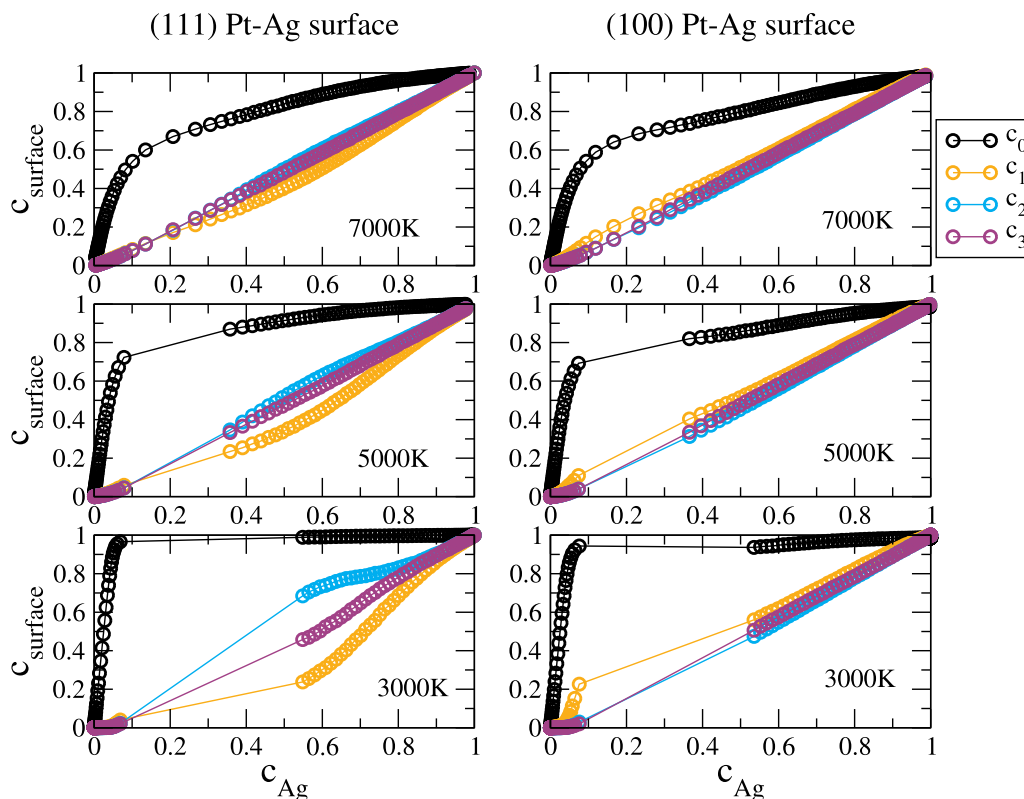
Fig. 8. Segregation isotherms at (111) and (100) surfaces at 7000K, 5000K and 3000K where we plot the top surface c_0 , the subsurface c_1 and the following c_2 and c_3 atomic layers concentrations in silver by increasing (up) or decreasing (down) the chemical potential.
