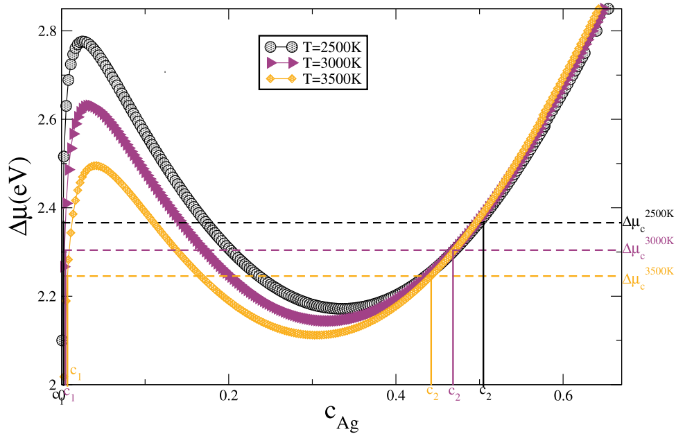
Fig. 4. Characterization of the critical concentrations c_1 and c_2 at high temperature from the canonical Monte Carlo simulations using virtual permutations.
