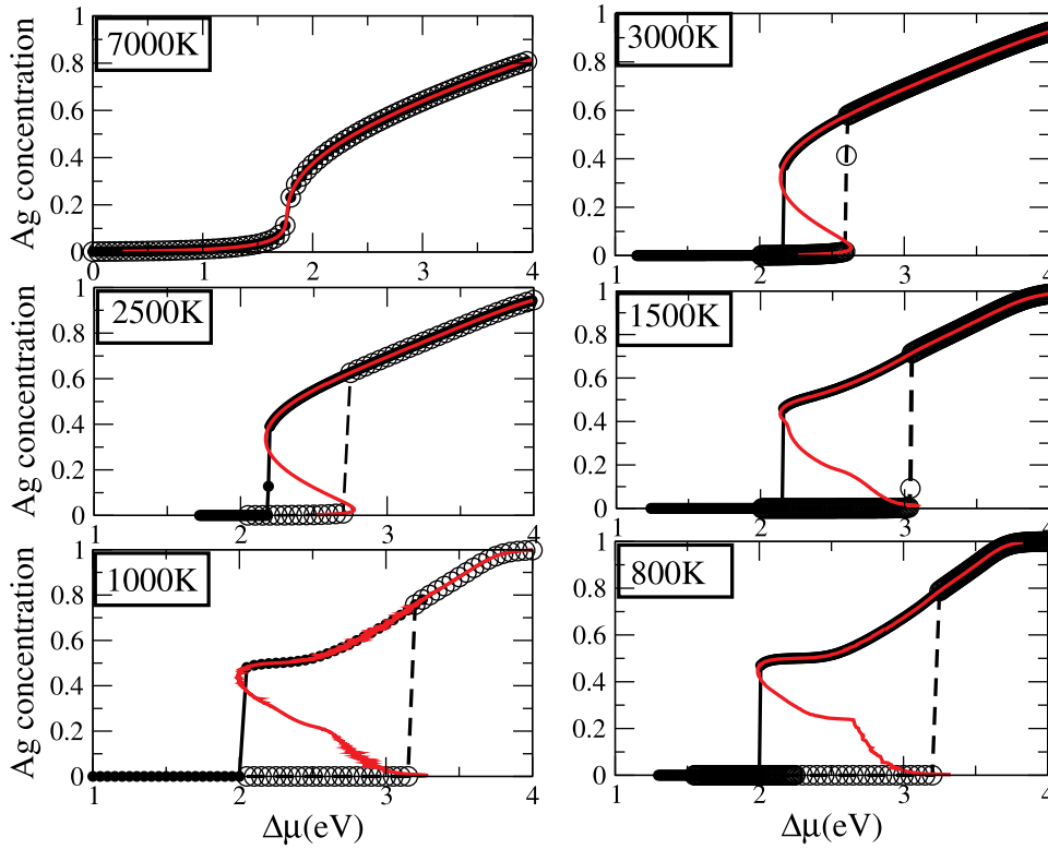
Fig. 3. Bulk isotherms determined via semi-grand canonical Monte Carlo simulations with increasing (dashed line) and decreasing (straight line) \Delta\mu from pure Pt metal (on the left) to pure Ag metal (on the right) or via canonical Monte Carlo simulation using the Widom method (virtual permutations) (red line). (For interpretation of the references to color in this figure legend, the reader is referred to the web version of this article.)
