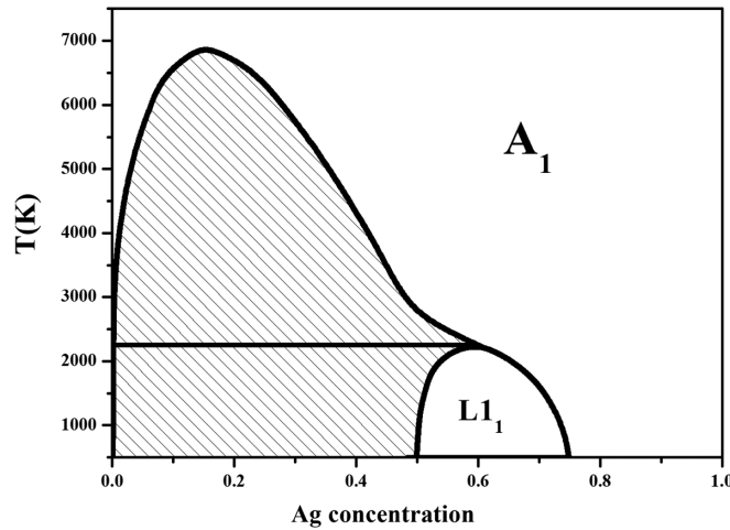
Fig. 7. Theoretical bulk phase diagram with the TBIM model and variable EPIs.
