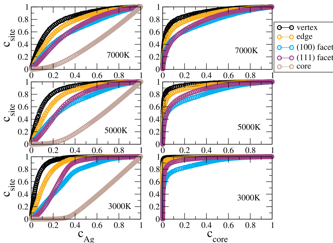
Fig. 11. Segregation isotherms of TOh 1289 cluster at high temperature for each different surface sites (vertex, edge, (111) and (100) facets) and core sites, and for up and down simulations (which are superimposed) with the same symbols as for the surfaces. In the first line the site concentrations are plotted as a function of the global silver concentration ( c_{Ag} ) and in the second line the same site concentration are plotted as a function of the core concentration in silver ( c_{core} ).
