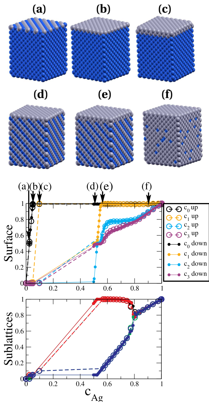
Fig. 10. Segregation isotherms of (100) surface at 300 K. The same as Fig. 9 with (a) for a concentration of 2.5%, (b) 5%, (c) 10%, (d) 50%, (e) 55% and (f) 90%.
