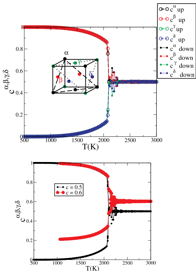
Fig. 5. Bulk sublattices from canonical Monte Carlo simulations at equiconcentration (top graph) and c=0.6 (bottom graph) with increasing (up) and decreasing (down) temperature. The sublattices are defined relatively to the (111) crystallographic planes. The L1_1 phase is characterized by the sublattices occupied two by two by Ag or Pt atoms. The disordered A1 solid solution is characterized by the four sublattices equally occupied.
