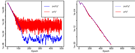
Figure 1: Trajectory of FedEM vs the number of epochs (left; blue line: \|h(\hat{S}^k)\|^2 ; red line: \|H_k\|^2 ) and of VR-FedEM (right; dashed blue line: \|h(\hat{S}^k)\|^2 ; solid red line: \|H_{t,k}\|^2 ).
