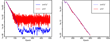
Figure 1: Trajectory of FedEM vs the number of epochs (left; blue line: \|\widehat{h}(\widehat{S}^k)\|^2 ; red line: \|H_k\|^2 ) and of VR-FedEM (right; dashed blue line: \|\widehat{h}(\widehat{S}^k)\|^2 ; solid red line: \|H_{t,k}\|^2 ).
