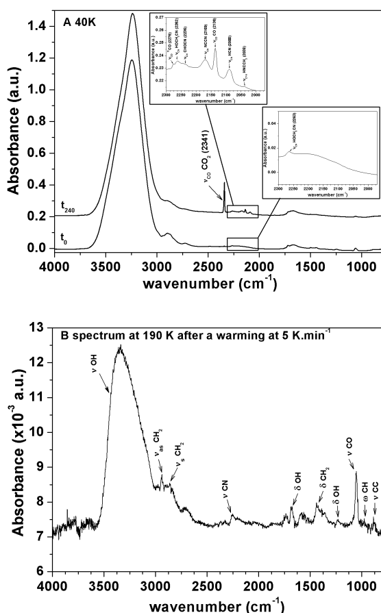
Fig. 7. UV irradiation of \text{HOCH}_2\text{CN} diluted in a water ice (1:10 \text{HOCH}_2\text{CN}:\text{H}_2\text{O} ). A ) Infrared spectra monitored after the \text{H}_2\text{O}:\text{HOCH}_2\text{CN} ice formation at 40 K, t_0 , and after 240 min of VUV irradiation at 40 K, t_{240} . B ) Infrared spectrum obtained at 190 K after the warming of the sample displayed in A ) t_{240} with a 5 \text{ K min}^{-1} temperature ramp. Note: vibration mode: stretching ( \nu ), bending ( \delta ), rocking ( \rho ), torsion ( \tau ), wagging ( \omega ). Type of vibration mode: asymmetric (as), symmetric (s).
