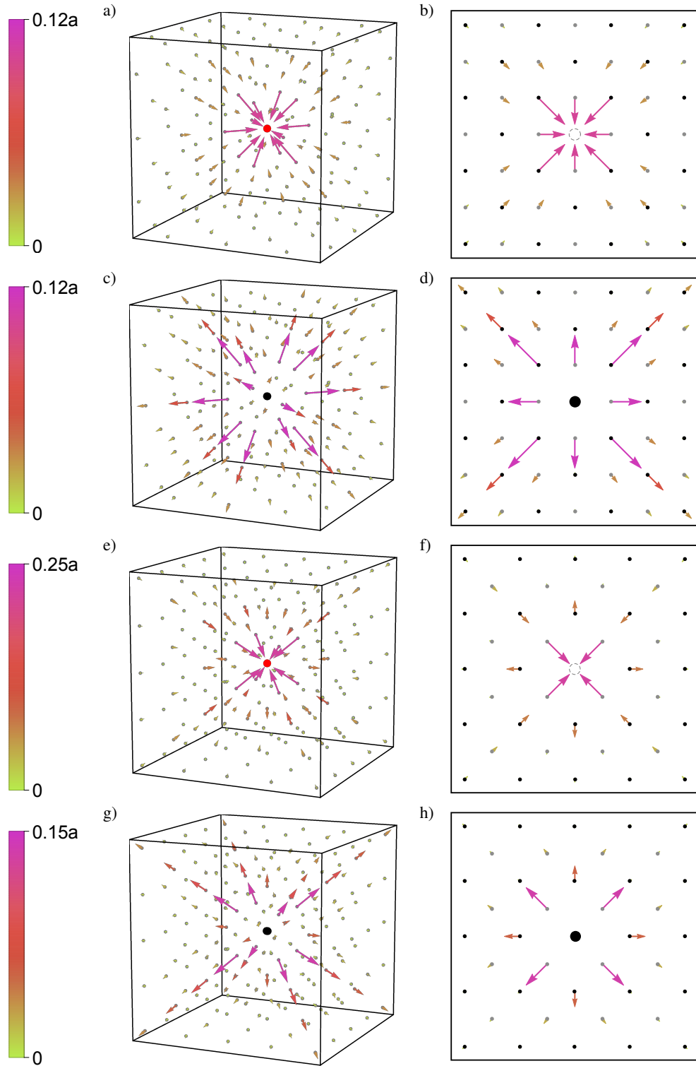
FIG. 2. Average lattice deformation due to a point defect in a-d) the FCC crystal at \kappa = 3.5 and \Gamma = 2565 and e-h) the BCC crystal at \kappa = 3.5 and \Gamma = 2400 . a-b,e-f) Deformation due to a vacancy (indicated by red or a dotted sphere) and c-d,g-h) deformation due to an interstitial (indicated by a black sphere). Left: 3d representation of part of the simulation box. The gray points represent the lattice sites. Right: projection of the displacement vectors on two (100) planes on top of each other. The black points represent the lattice sites that lie in the plane of the defect and the gray points the lattice sites in the neighboring plane. In all figures the size of the arrows is exaggerated, but the color of the arrows indicates the deformation in terms of the Wigner Seitz radius a .
