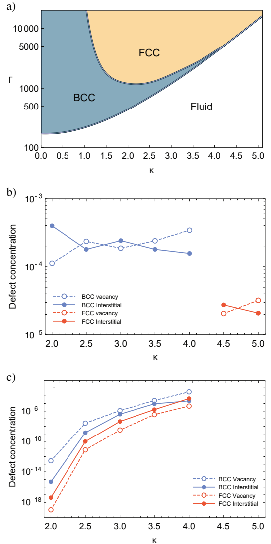
FIG. 1. a) Phase diagram of Yukawa systems in the (\kappa, \Gamma) plane, with the phase boundaries from Refs. 6 and 7. Vacancy and interstitial concentrations plotted along b) fluid-crystal phase boundary and c) BCC-FCC phase boundary. We estimate an error of up to 0.2k_B T in our calculation of the \mu^{\text{vac(int)}} , leading to an approximate error of a factor of 1.2 in the concentrations.
