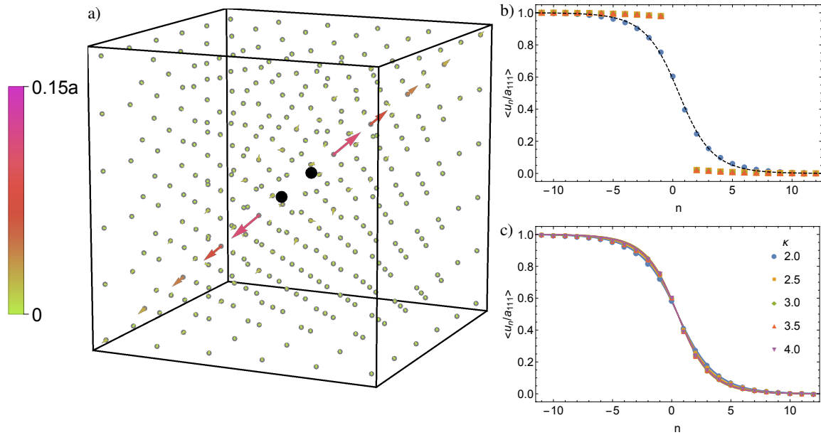
FIG. 3. a) Lattice deformation due to an interstitial in the BCC crystal at \kappa = 3.5 and \Gamma = 2400 . The gray points represent the lattice sites of part of the simulation box and the black spheres represent the positions of the interstitial and its companion. The size of the arrows is exaggerated, but the color of the arrows indicates the deformation in terms of the Wigner Seitz radius a . Note that these deformations are averaged over multiple configurations which have been rotated so that the defect always points along the same direction. b) Displacement u_n along the four (111) directions for the same system as a). The blue dots indicate u_n along the direction of the crowdion and the dashed line represents the corresponding fitted soliton solution. c) u_n along the direction of the crowdion for \kappa = 2.0 and \Gamma = 1000, 1100, 1205 (blue dots), \kappa = 2.5 and \Gamma = 1000, 1100, 1205 (yellow squares), \kappa = 3.0 and \Gamma = 1205, 1400, 1600 (green diamonds), \kappa = 3.5 and \Gamma = 2200, 2300, 2400 (orange triangles), \kappa = 4.0 and \Gamma = 4000, 4100, 4200 (purple triangles). The lines represent the corresponding fitted soliton solutions.
