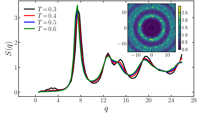
FIG. 4. Structure factor of the 12-patch system corresponding to temperatures where the system has not crystallized. The inset shows the projection of the structure factor in the xy -plane at T = 0.3 .
