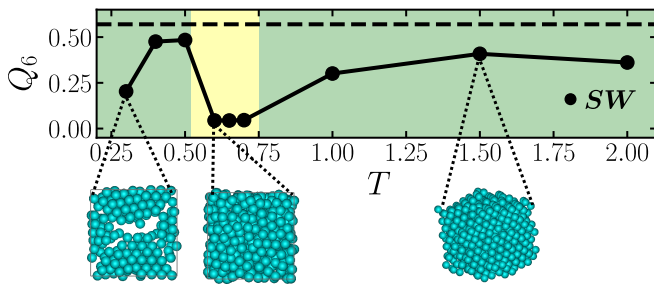
FIG. 1. Q_6 as a function of temperature for a monodisperse of square well at packing fraction \eta = 0.56 . Yellow regions correspond to a fluid phase and green regions to a crystallized phase. The dashed line is the Q_6 value of a perfect FCC lattice. Below each region we illustrate the phase with a corresponding snapshot. Note that at the lowest temperature we see signs of phase separation.
