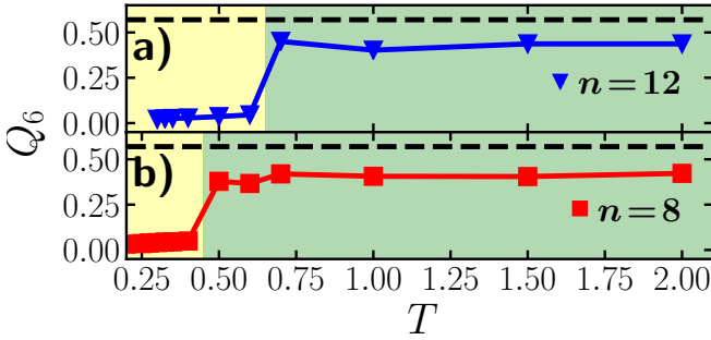
FIG. 3. Q_6 as a function of temperature for the two patchy cases a) n = 12 patches and b) n = 8 patches at a packing fraction corresponding to \eta = 0.56 . Yellow regions correspond to a fluid phase and green regions to a crystallized phase, dashed line is the Q_6 value of a perfect FCC lattice.
