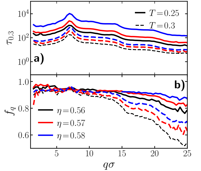
FIG. 12. a) Collective relaxation time as a function of q -vector. Continuous lines correspond to T = 0.25 and dashed lines to T = 0.3 , different colors correspond to different packing fractions \eta . b) Corresponding non-ergodicity parameter.
