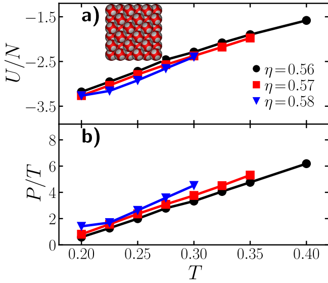
FIG. 7. a) Average energy per particle as a function of temperature of the n = 8 patches. Inset shows a fully bonded face-centered cubic crystal structure at close packing. Each particle is bonded to eight neighbors. b) Dimensionless pressure, note that at temperatures lower than the ones studied here ( T \approx 0.18 or lower) the system might present phase separation.
