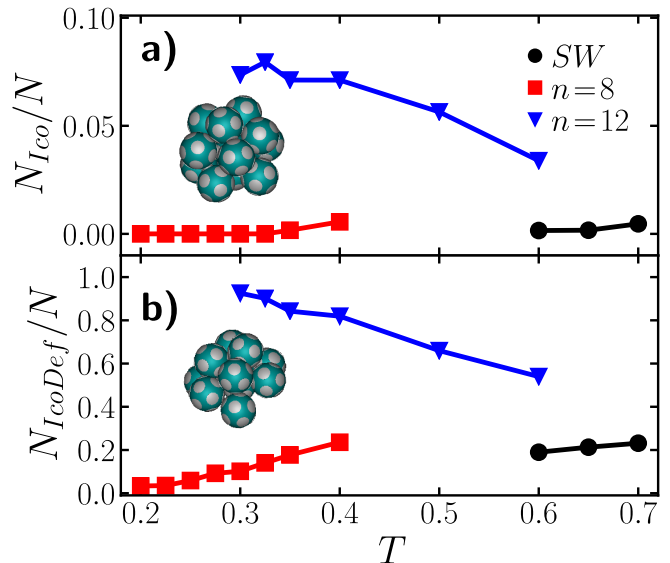
FIG. 6. a) Fraction of particles in an icosahedral cluster as a function of temperature for the temperatures where the system is a fluid. b) Fraction of particles in a defective icosahedral cluster. The inset shows an illustration of the icosahedral and defective icosahedral cluster respectively.
