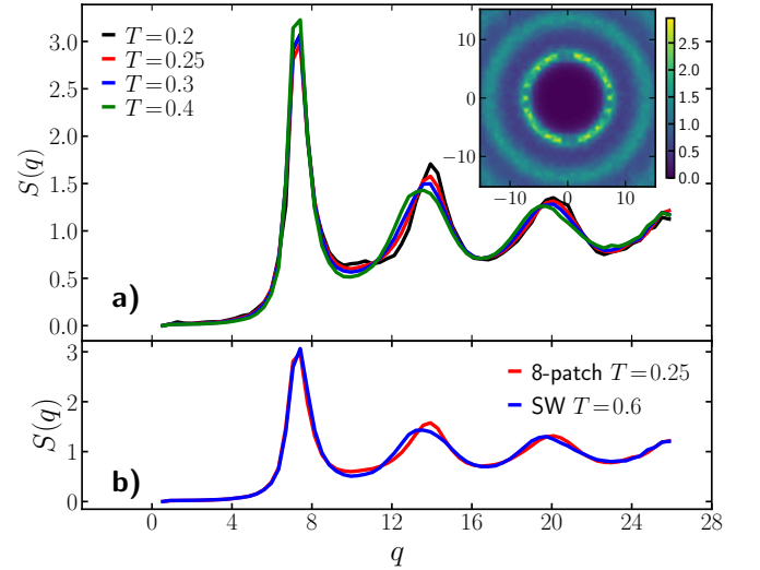
FIG. 5. a) Structure factor of 8-patch fluids. The inset shows the two-dimensional structure factor in the xy -plane at T = 0.3 . b) Comparison between S(q) of the 8-patch system and a SW liquid.
