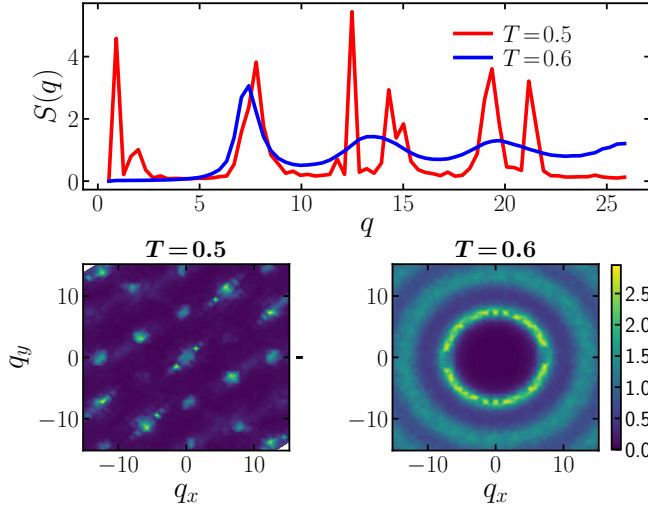
FIG. 2. a) Structure factor of the square well system with potential range of r_c = 1.03\sigma of a crystallized system at T = 0.5 and a liquid system at T = 0.6 . b) Projection of the structure factor of the same crystallized system in the plane xy . c) Projection for the corresponding liquid state.
