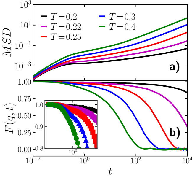
FIG. 9. a) Mean-squared displacement of the 8-patch fluid at a fixed packing fraction \eta = 0.56 . b) Corresponding Intermediate Scattering Function. The inset shows a close-up of the region where the first decay in the ISF happens.
