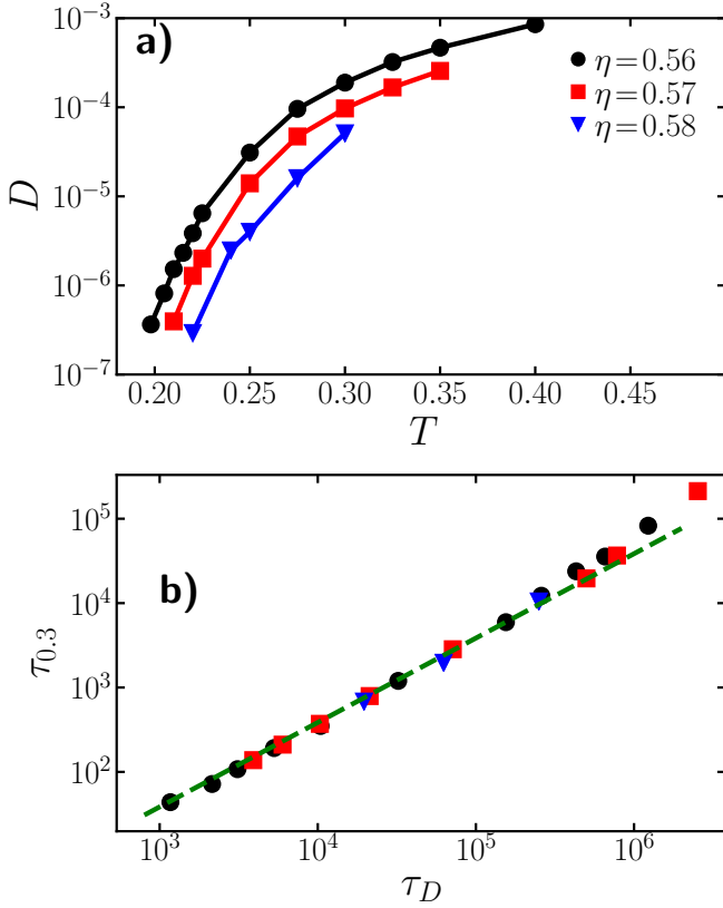
FIG. 11. a) Dimensionless diffusion of the n=8 patch for different packing fractions. b) Relaxation times \tau_{0.3} as a function of the diffusion time \tau_D .
