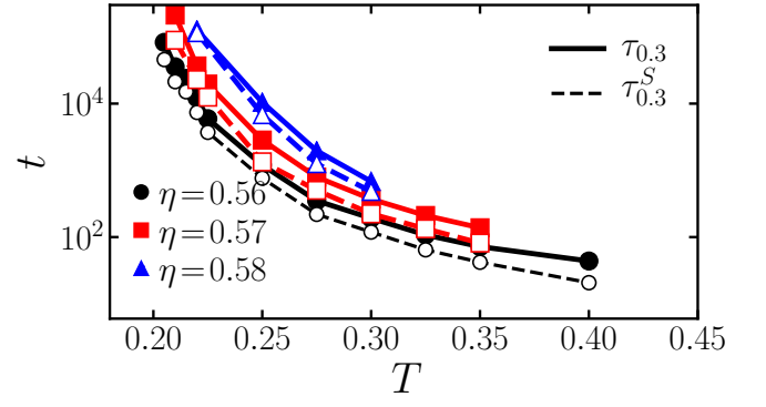
FIG. 10. Relaxation times of the n=8 case for all the investigated packing fractions. Dashed lines and empty symbols correspond to the ones extracted from the self intermediate scattering function and continuous lines to the collective one. Both set of data refer to q\sigma = 7.1 .
