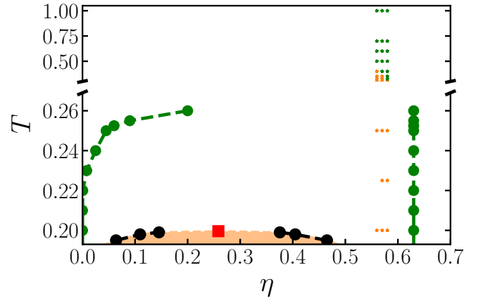
FIG. 8. Phase diagram of the 8-patch system. The gas-liquid region, obtained from Successive Umbrella Sampling simulations, is colored in orange. The coexisting densities are marked by black filled circles and the location of the critical point by a red filled square. The low-temperature gas-crystal coexistence, estimated from direct coexistence simulations, is denoted with green circles. Green stars correspond to simulations where the system crystallizes and orange ones to simulations in the fluid phase.
