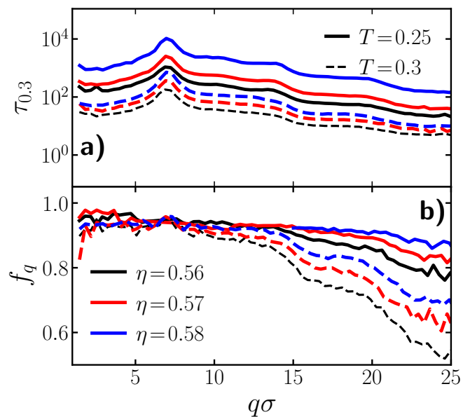
FIG. 12. a) Collective relaxation time as a function of q -vector. Continuous lines correspond to T = 0.25 and dashed lines to T = 0.3 , different colors correspond to different packing fractions \eta . b) Corresponding non-ergodicity parameter.
