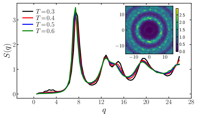
FIG. 4. Structure factor of the 12-patch system corresponding to temperatures where the system has not crystallized. The inset shows the projection of the structure factor in the xy -plane at T = 0.3 .
