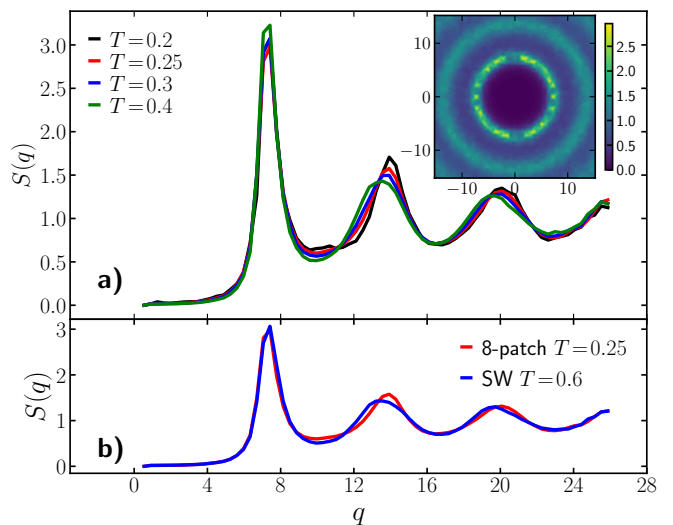
FIG. 5. a) Structure factor of 8-patch fluids. The inset shows the two-dimensional structure factor in the xy -plane at T = 0.3 . b) Comparison between S(q) of the 8-patch system and a SW liquid.
