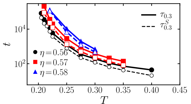
FIG. 10. Relaxation times of the n=8 case for all the investigated packing fractions. Dashed lines and empty symbols correspond to the ones extracted from the self intermediate scattering function and continuous lines to the collective one. Both set of data refer to q\sigma = 7.1 .
