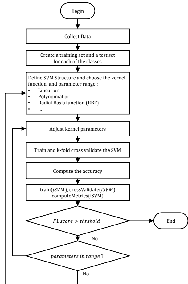
Fig. 8: Kernel-selection algorithm.
