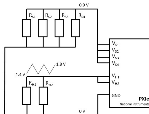
Fig. 2: Electrical configuration of the sensor: RS1, RS2, RS3 and RS4 are the resistances of the four detection zones. RH1 and RH2 are heating resistances of the two heaters [31].
