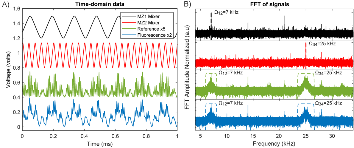
Figure 3: A: Time domain signals acquired for phase-modulated rapid-scanning fluorescence-detected 2DES. These signals are: mixer signals for MZ1 and MZ2, the four-pulse reference signal for interferometric tracking of the time delays and the four-pulse fluorescence signal. The signals are offset for clarity. (Note that a small subset of the full scan is shown). B) Fourier transform of the time domain signals shown in A, indicating the frequencies at which different signals appear. Also shown are the filter functions used to extract the quantities of interest.
