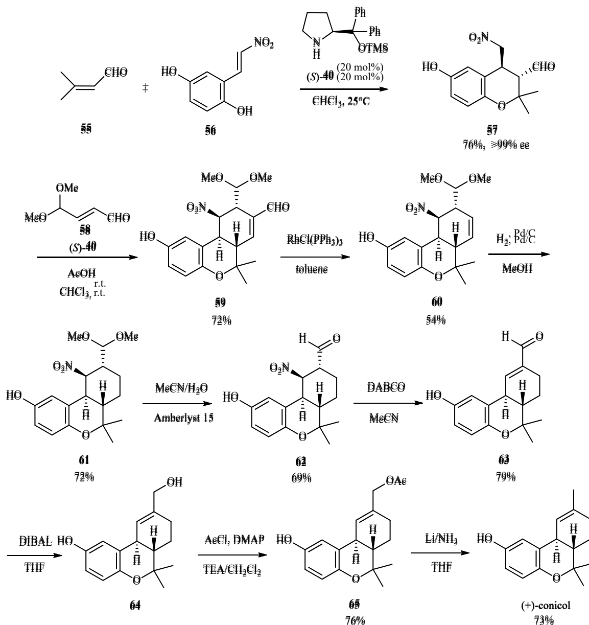
Scheme 7. Synthesis of (+)-conicol.
