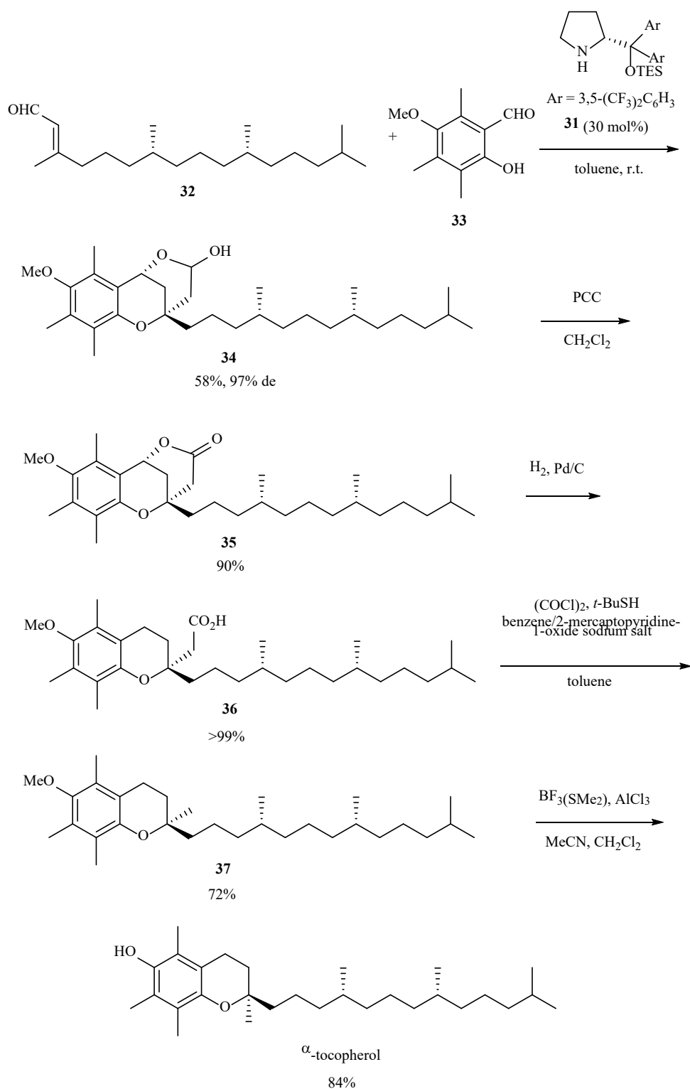
Scheme 4. Synthesis of α-tocopherol.
