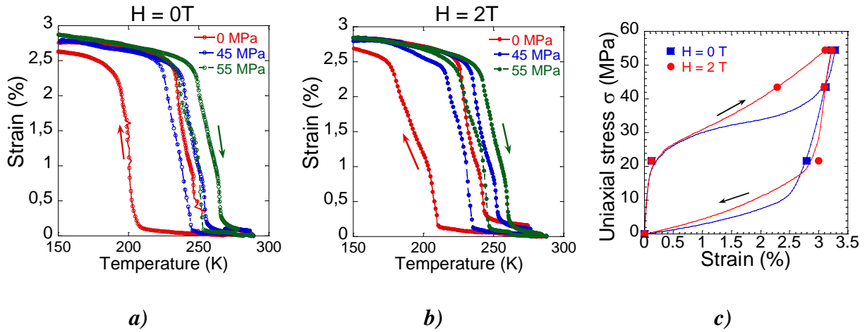
Figure 9: Strain as a function of temperature ( \epsilon -T curves) measured during cooling and heating under different constant uniaxial stress levels for H = 0 (a) and H = 2 T (b). Effect of the magnetic field on stress – strain response at 220 K (c).
