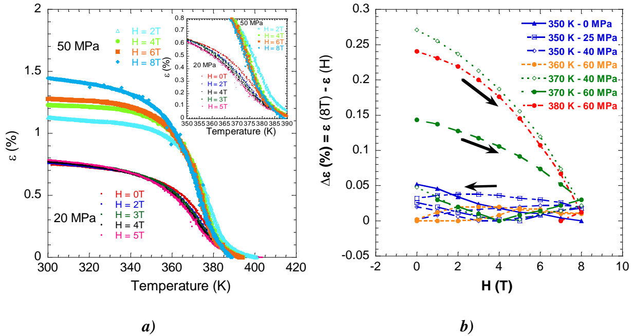
Figure 10 : a) Strain versus temperature increase in a Ni_{45}Co_5Mn_{37.5}In_{12.5} single crystal uniaxially compressed under 20 and 50 MPa. In inset a magnification of the \varepsilon(T) curves shows the decrease of the transformation temperature under magnetic field increase. b) Magnetic field induced strain variation in the single crystal uniaxially compressed under 0, 25 and 40 MPa at 350 K (blue curves), under 60 MPa at 360 K (orange curve), under 40 and 60 MPa at 370 K (green curves) and under 60 MPa at 380 K (red curve).
