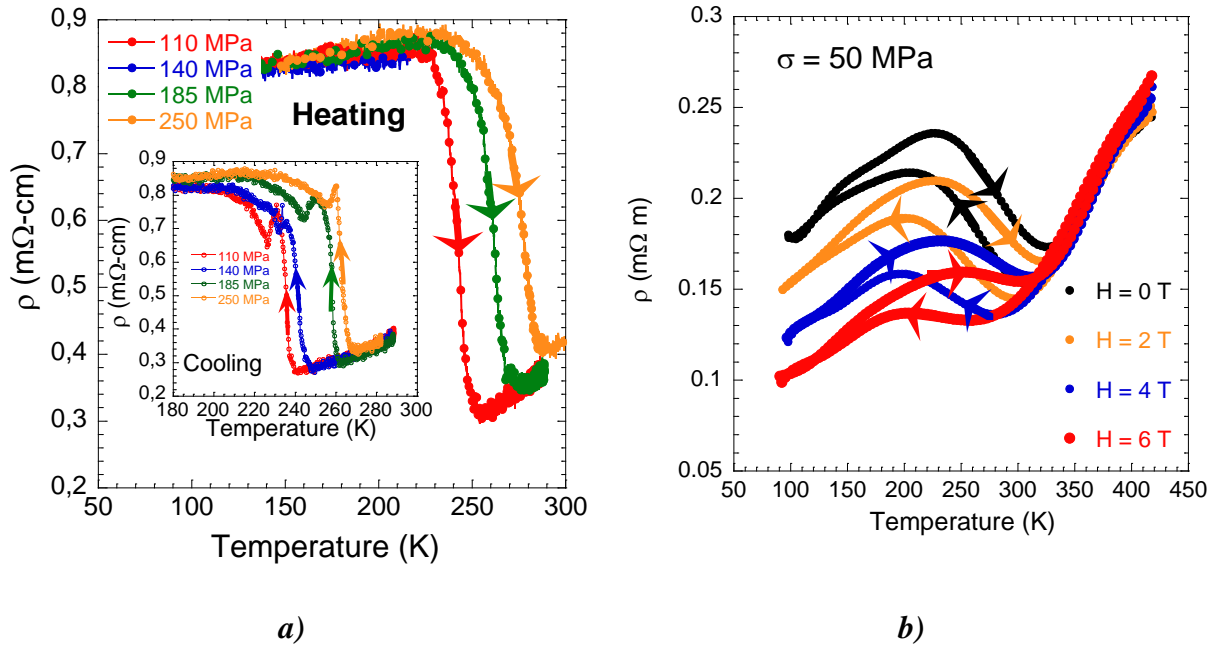
Figure 8: Temperature dependence of the electrical resistivity under uniaxial stress varying between 110 MPa and 250 MPa (a) and under magnetic field varying between 0 T and 6 T (b) for a Ni_{50}Mn_{34.5}In_{15.5} single crystal.
