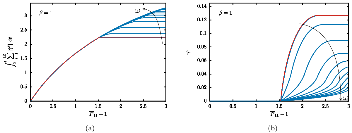
Fig. 4. Influence of material parameter \omega on the post-coalescence regime of void growth and void coalescence plastic slip variables. \omega varies from 1.5 to 100 GPa and \beta is fixed to 1. \sigma_s^e = 615 MPa in this example.
