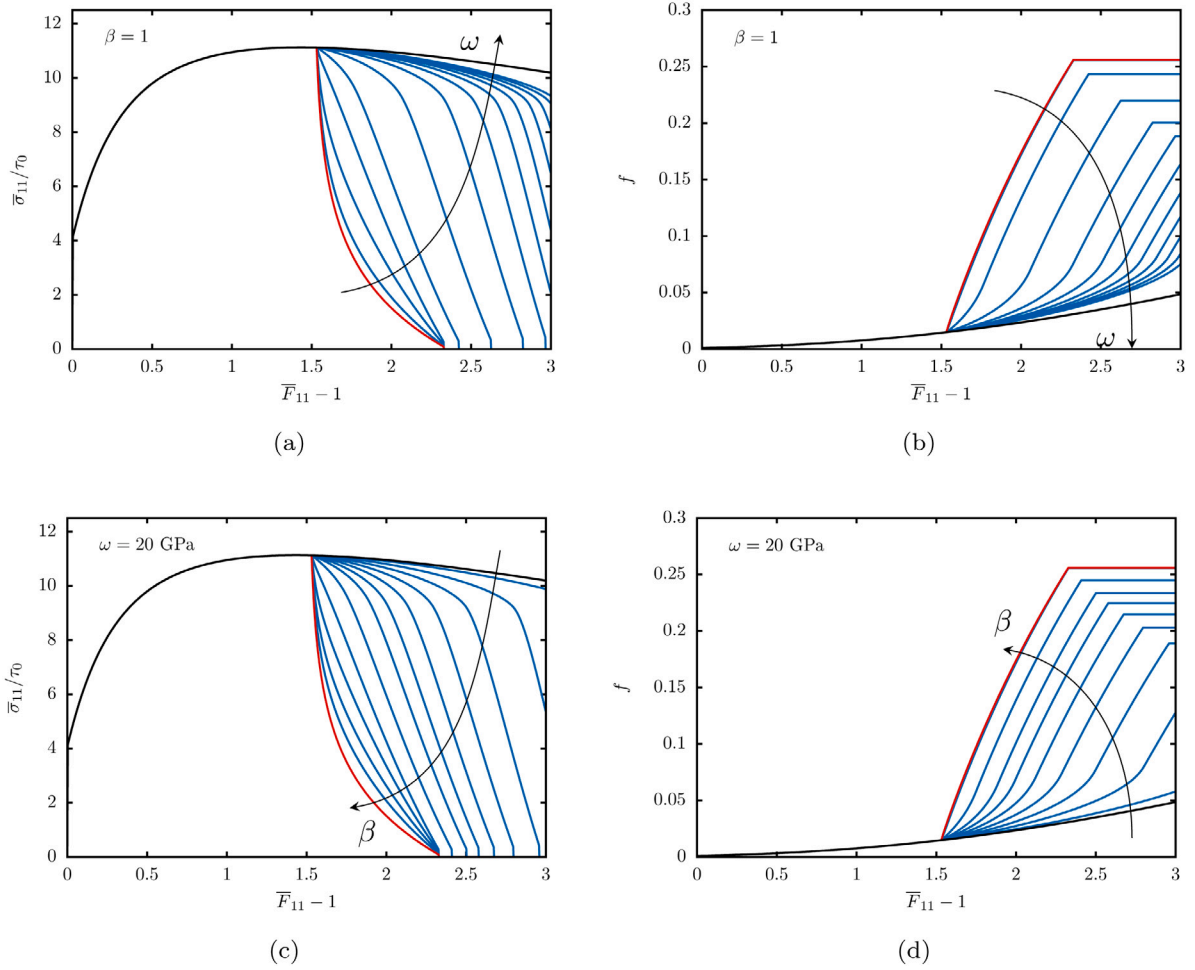
Fig. 3. Influence of material parameters \omega and \beta from Eq. (46) on the post-coalescence regime of the tensile stress and the porosity. \omega varies from 1.5 to 100 GPa and \beta varies from 0.1 to 10. \sigma_s^e = 615 MPa in this example.
