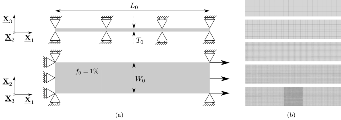
Fig. 5. (a) Sketch of the plate geometry and applied plane strain boundary conditions. (b) Finite element meshes used in the mesh convergence analysis. From top to bottom, meshes are respectively composed of 80, 320, 1280, 5120 and 13184 elements.
