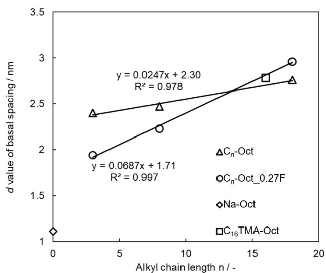
Figure 4. Relationships between the number of carbon atoms in alkyl chain and d values of basal spacing of C_n -Oct and C_n -Oct_0.27F.
