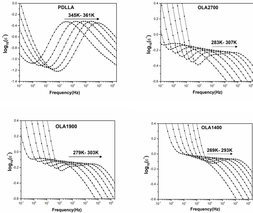
Figure 2: Frequency dependence of the imaginary part of complex permittivity \epsilon'' at several temperatures in logarithmic scale for PDLLA, OLA2700, OLA1900, and OLA1400.
