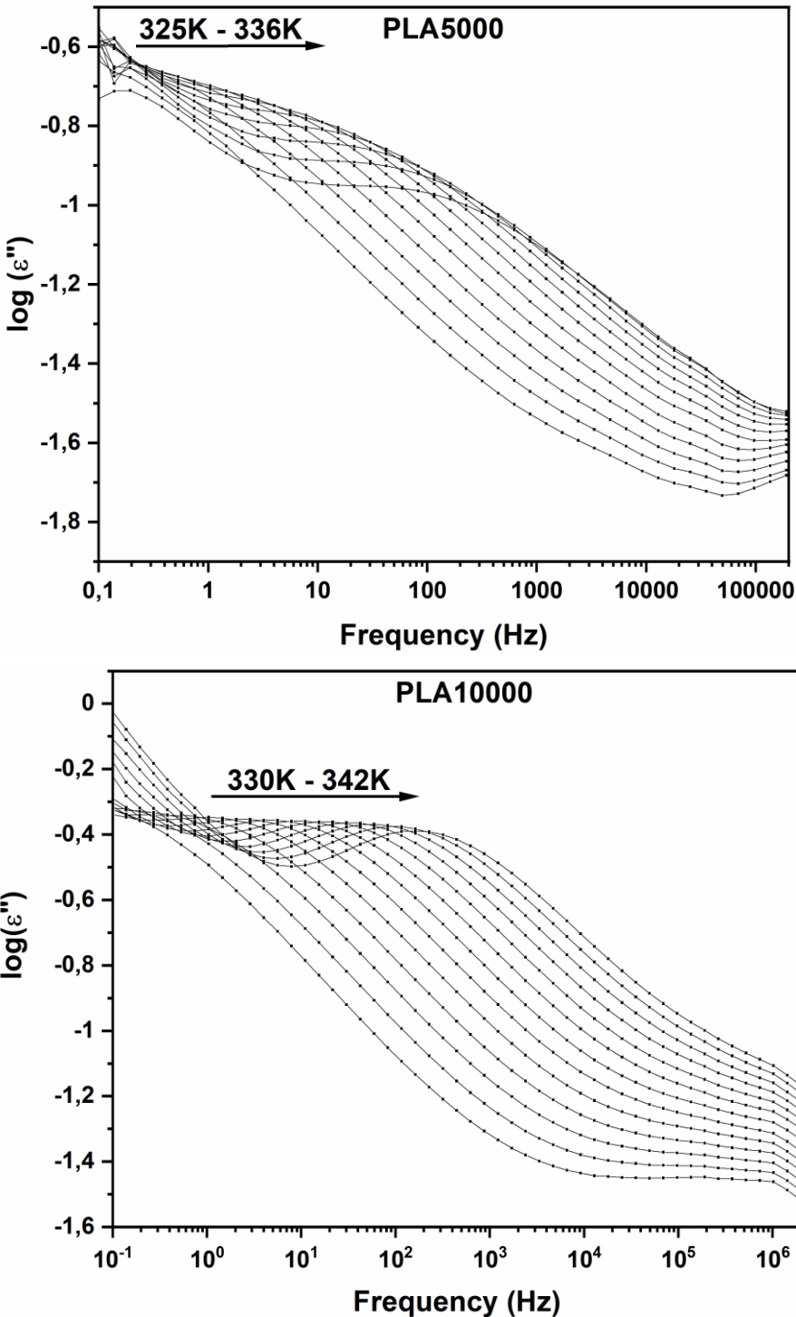
Figure SI4: Frequency dependence of the imaginary part of the complex permittivity \epsilon'' at several temperatures in logarithmic scale for PLA5000 and PLA10000.
