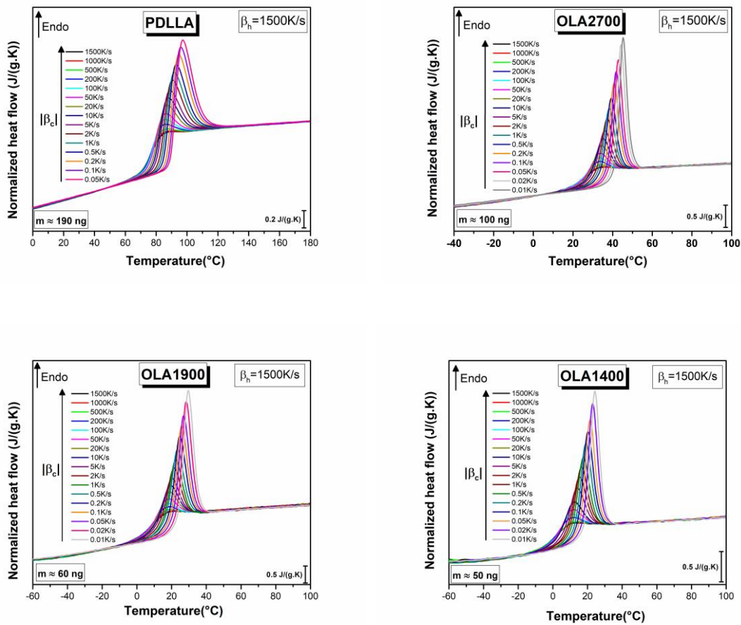
Figure 5: FSC normalized heat flow of amorphous PDLLA and OLAs for various cooling rate |\beta_c| (ranging from 0.01 K/s up to 1500 K/s) at constant heating rate \beta_h = 1500 K/s. The sample masses have been estimating by comparing the \Delta C_p step values obtained by MT–DSC and FSC. [8]
