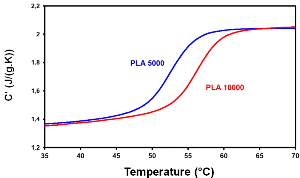
Figure SI3: MT-DSC reversing heat capacity signal recorded in the glass transition range for amorphous PLA5000 and PLA10000.
