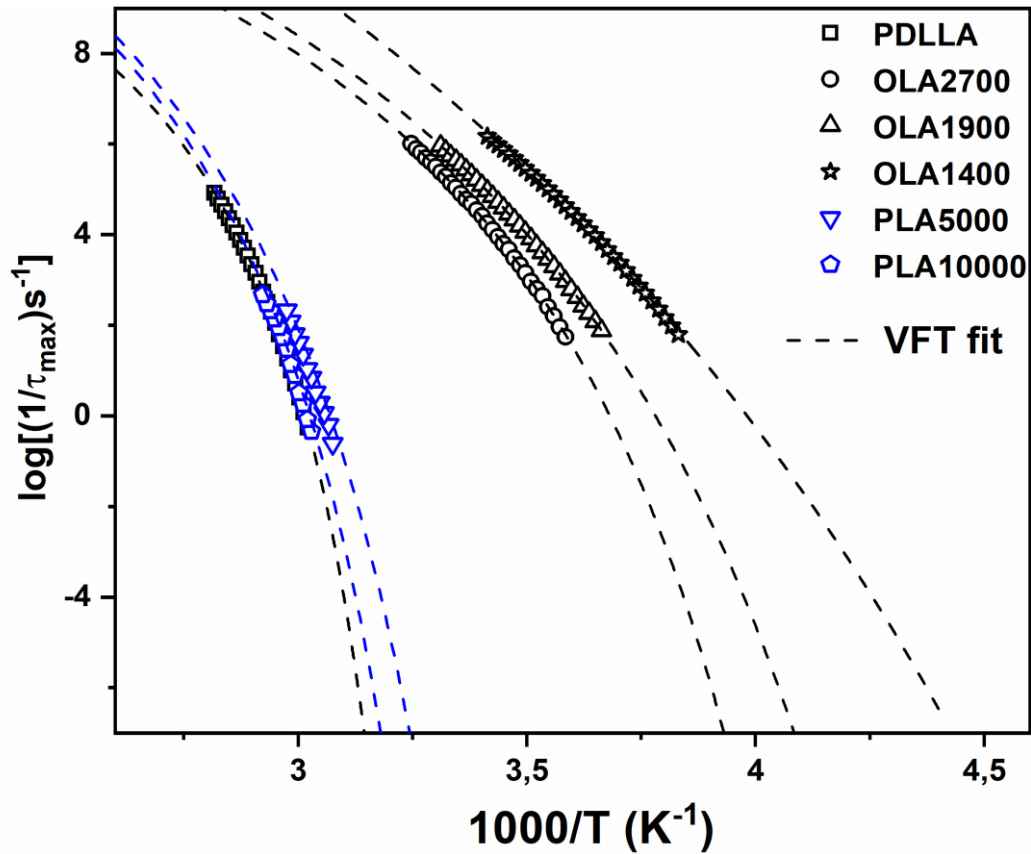
Figure SI.5: Temperature dependence of the relaxation rate ( 1/\tau_{max} ) determined from DRS for PLA5000 (blue triangles) and PLA10000 (blue pentagons). Results obtained for PDLLA (black squares), OLA2700 (black circles), OLA1900 (black triangles) and OLA1400 (black stars) are added. The dashed curve is the VFT fit of the experimental data.
