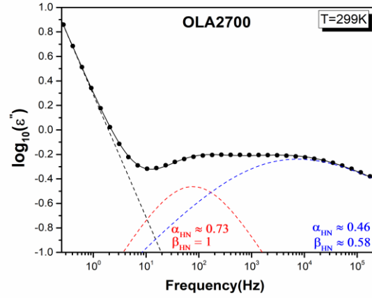
Figure 3: Fitting procedure used to investigate the segmental relaxation region with a conductivity contribution (black dashed line) and two Havriliak–Negami complex functions: one for the low frequency process (red dashed line) and another for the \alpha –relaxation (blue dashed line). The black solid line is the final fitting. The Havriliak–Negami shape parameters \alpha_{HN} and \beta_{HN} are also reported. This example concerns the dielectric response of OLA2700 recorded at 299 K.
