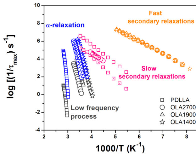
Figure 4: Relaxation map including all the relaxation processes recorded from DRS measurements for PDLLA, OLA2700, OLA1900, and OLA1400.
