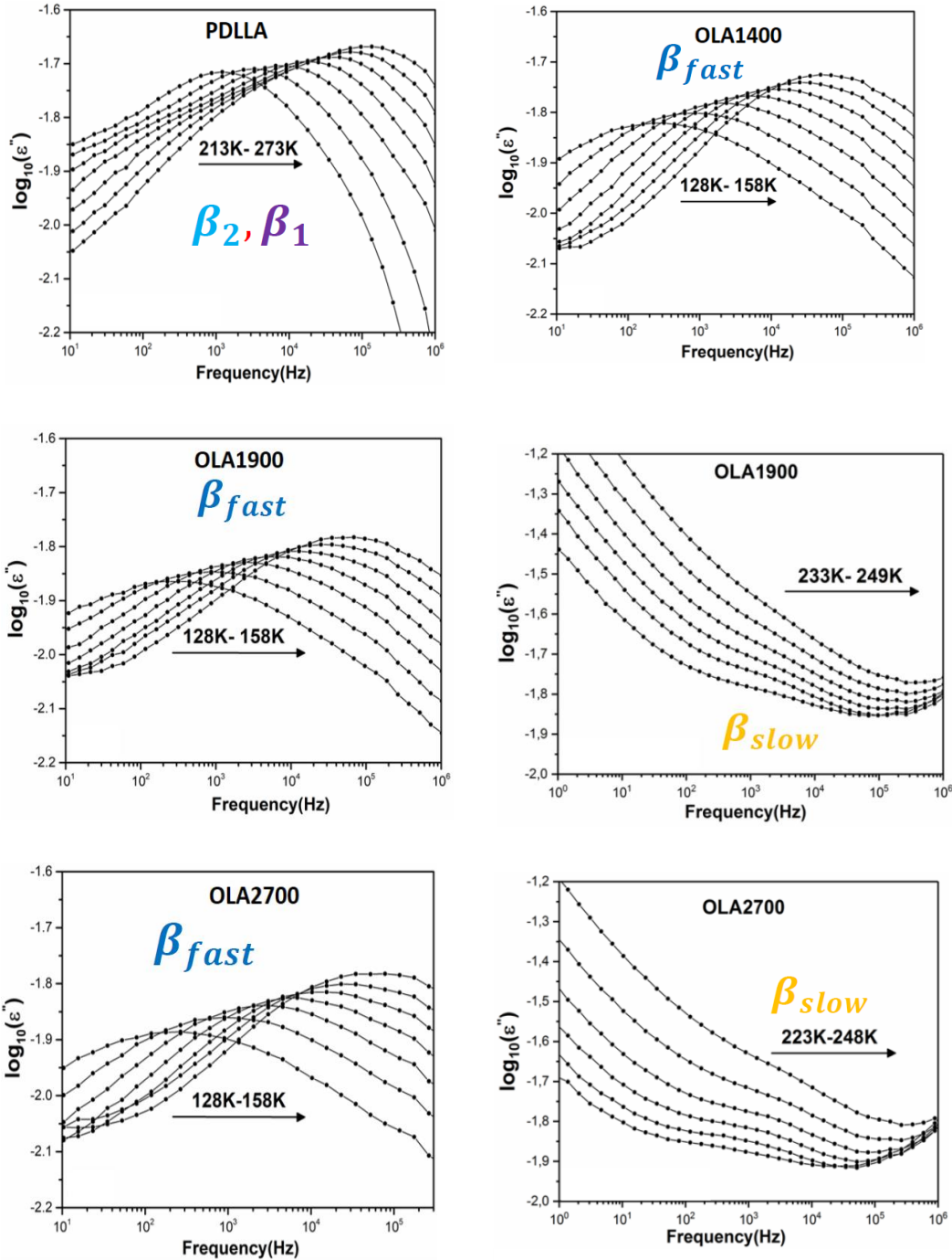
Figure SI.1: DRS signatures of local relaxation processes recorded for PDLLA and OLAs.
