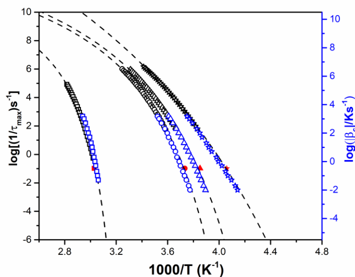
Figure 6: Temperature dependence of the relaxation rate ( 1/\tau_{max} ) (left coordinate) and cooling rate |\beta_c| dependence of T_g' (right coordinate), determined from DRS (black symbols), MT–DSC (red symbols) and FSC (blue symbols) respectively, for PDLLA (squares), OLA2700 (circles), OLA1900 (triangles) and OLA1400 (stars). Dashed line is VFT fit to all data obtained from FSC+DRS. The glass transition temperature T_g from MT–DSC is defined at \tau = 10 s which approximately corresponds to a 60s period.
