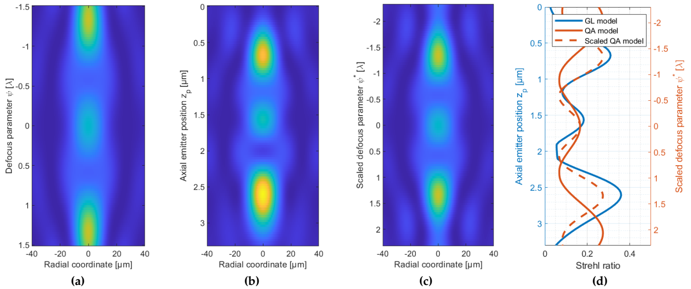
Fig. 6. (a) PSF profile as a function of the defocus parameter \psi \in [-1.5\lambda, 1.5\lambda] using the QA model. (b) PSF profile as a function of the emitter position z_p with the GL model ( n_i = 1.52 and n_s = 1.33 ). (c) PSF profile as a function of the equivalent defocus parameter \psi^* using the QA model. (d) Variation of the Strehl ratio for the optical systems illustrated in (a), (b) and (c). The microscope is equipped with the phase mask illustrated in Fig. 3 and its configuration and the simulation parameters are described in Table 1.
