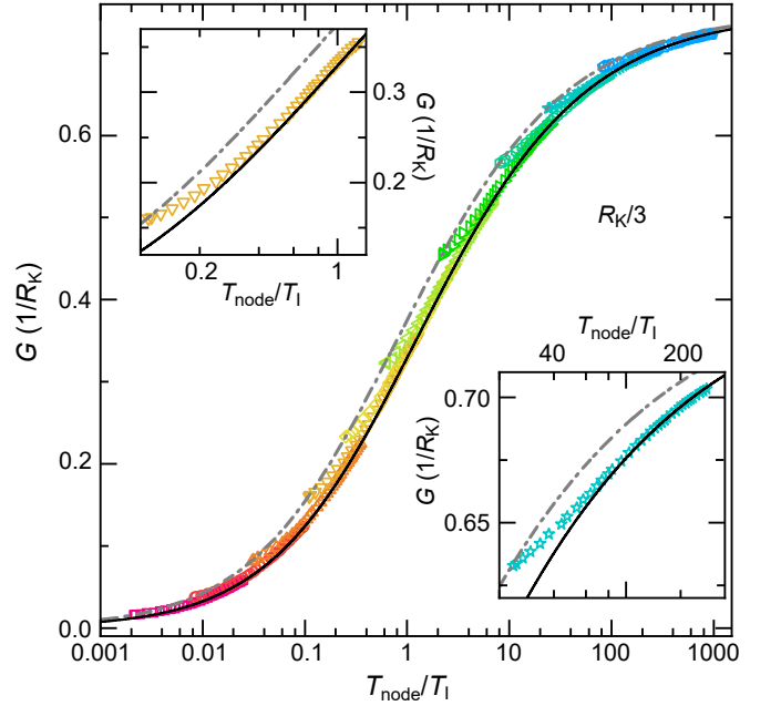
FIG. 5. Conductance for arbitrary channel tunings and R = R_K/3 versus node temperature. Open symbols: measured sample conductance G at T \simeq 8 mK versus heated-up T_{\text{node}} . Different tunings ( \tau_\infty ) of the channel are shown using different symbols and colors. For each tuning a unique value of T_1 is determined by matching the lowest temperature data point at T_{\text{node}} \simeq T \simeq 8 mK with G_{1/3}^{\text{eq}}(T/T_1) , the universal prediction at uniform temperatures (gray dash-dotted line). The black line corresponds to the universal prediction with the temperature reduction factor T_{\text{node}} \rightarrow \alpha T_{\text{node}} predicted to apply for large temperature bias in the tunnel regime ( \alpha \simeq 0.648 , see Appendix Eq. (18)). Insets: magnified view for intermediate channel tunings.
