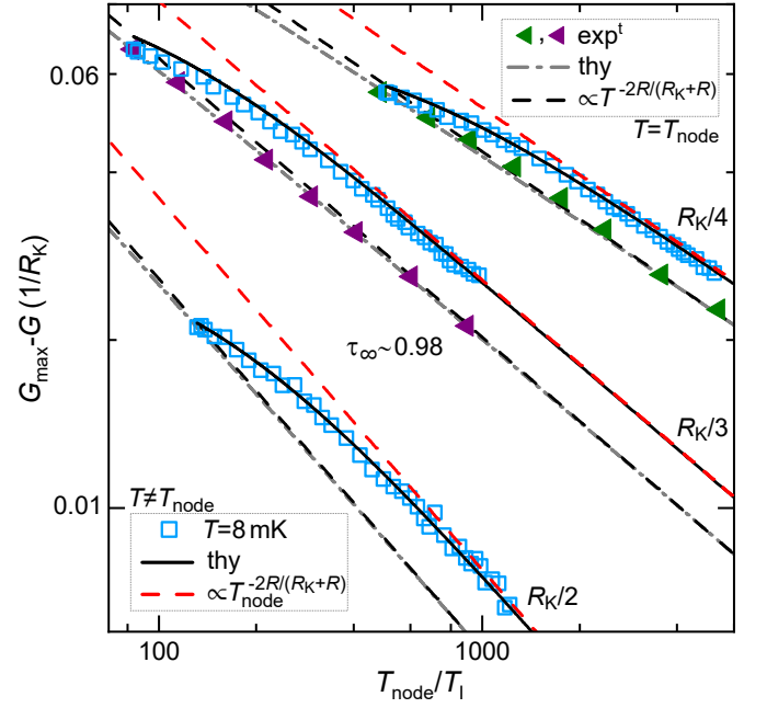
FIG. 4. Conductance versus node temperature in the near ballistic regime ( 1 - \tau \ll 1 ). The difference G_{\text{max}} - G , between ballistic limit G_{\text{max}} = \frac{N}{N+1} R_K^{-1} and sample linear conductance G(V \rightarrow 0) , is plotted in a log-log scale as a function of the rescaled node temperature T_{\text{node}}/T_1 for R = R_K/2 , R_K/3 and R_K/4 . Gray dash-dotted lines: full universal predictions at uniform temperatures ( T_{\text{node}} = T = T_{\text{env}} ) [35]. Black and red dashed lines: asymptotic ( G_{\text{max}} - G \rightarrow 0 ) power law predictions at uniform temperatures (black) and in the limit T_{\text{node}} \gg T with T_{\text{env}} = T_{\text{node}}/2 (red). Black continuous lines: predictions for a near ballistic junction temperature biased at T_{\text{node}} \geq T with T = 8 \text{ mK} and T_{\text{env}} = (T + T_{\text{node}})/2 . Full and open symbols: measurements at a uniform temperature T \simeq T_{\text{node}} (full) and in the presence of a temperature bias at fixed T \simeq 8 \text{ mK} (open), respectively. The scaling temperature T_1 is set by adjusting to the universal theory the lowest temperature point T_{\text{node}} \simeq 8 \text{ mK} .
