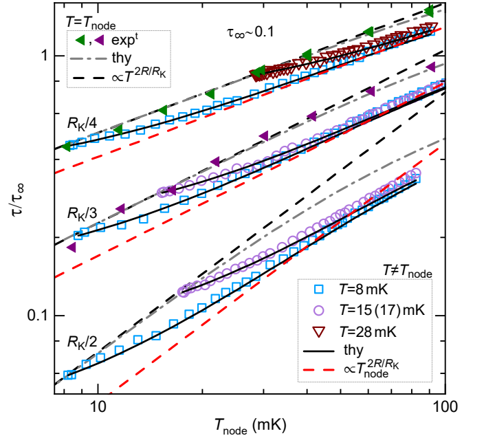
FIG. 3. Renormalized transmission probability versus node temperature in the tunnel regime ( \tau_{\infty} \ll 1 ) at low bias voltage ( V \rightarrow 0 ). Full symbols: experimental \tau/\tau_{\infty} at a uniform temperature ( T_{\text{node}} \simeq T \simeq T_{\text{env}} ) for R = R_K/3 (purple) and R_K/4 (green). Gray dash-dotted lines and black dashed lines: full and asymptotic ( k_B T \ll h/2\pi RC ) predictions, respectively, both of them for a uniform temperature T = T_{\text{node}} = T_{\text{env}} . Open symbols: renormalized transmission probability data obtained in the presence of the series resistances R = R_K/2 , R_K/3 and R_K/4 , with a temperature bias T_{\text{node}} - T \geq 0 developing from different fixed values of the temperature T . Black continuous lines and red dashed lines: full and asymptotic ( k_B T \ll k_B T_{\text{node}} \ll h/2\pi RC ) predictions, respectively, both of them versus T_{\text{node}} at fixed T and assuming an electromagnetic environment at T_{\text{env}} = (T + T_{\text{node}})/2 . For clarity, the data/theory are shifted vertically in this log-log plot by a factor of 2 (4) for R = R_K/3 ( R_K/4 ).
