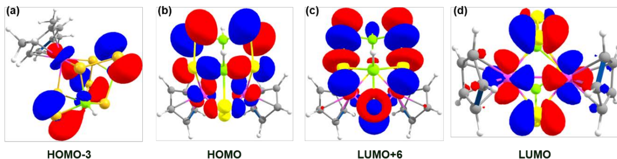
Fig. 5 Selected frontier molecular orbitals of tris-homocubane analogues 3 (a) and 4' (b, c) and bis-homocubane analogue 5' (d).
