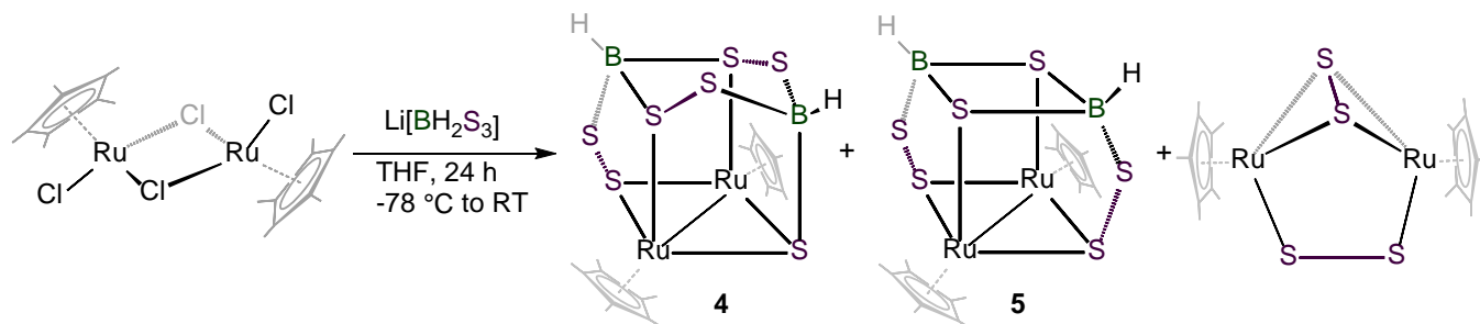
Scheme 2 Reaction of [\text{Cp}^*\text{Ru}(\mu\text{-Cl})\text{Cl}]_2 with \text{Li}[\text{BH}_2\text{S}_3] .
