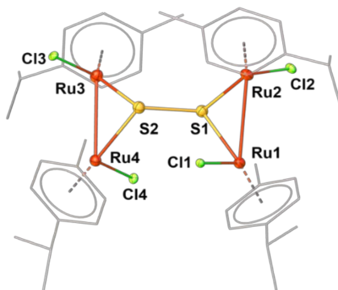
Fig. 1 Molecular structure of 1 . Selected bond lengths (Å) and angles (°) are: S1-S2 2.1089(8), Ru1-Ru2 2.9392(3), Ru3-Ru4 2.9395(4), Ru1-S1 2.3202(6), Ru2-S1 2.3350(6), Ru3-S2 2.3298(6), Ru4-S2 2.3150(6); Ru1-S1-Ru2 78.30(2), Ru4-S2-Ru3 78.52(2), S1-S2-Ru3 110.03(3), S1-S2-Ru4 115.03(3).
