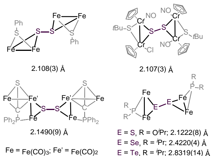
Chart 1. Selected examples of transition metal dichalcogenide complexes featuring an E–E bond (E = S, Se or Te). All the bond distances mentioned are the E–E bond distances.
