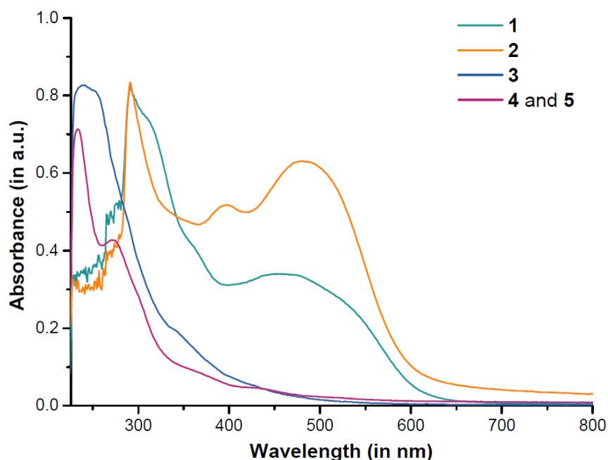
Fig. 6 Combined UV-vis spectra of 1 , 2 , 3 , 4 and 5 in \text{CH}_2\text{Cl}_2
