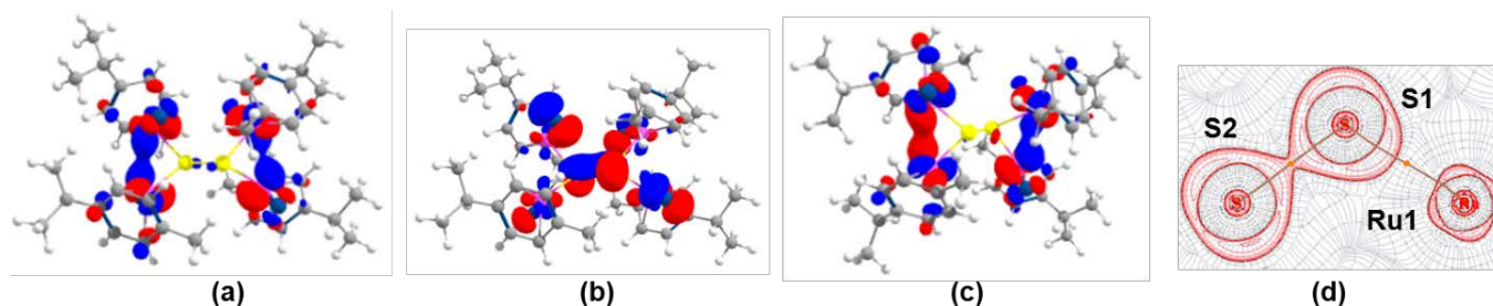
Fig. 2 (a) HOMO, (b) HOMO-13 and (c) LUMO of 1 . (d) Contour line diagram of Laplacian of electron density of 1 along the Ru–S1–S2 plane. Solid red lines specify areas of charge concentration ( \nabla^2\rho(r) < 0 ) and dashed black lines display areas of charge depletion ( \nabla^2\rho(r) > 0 ). Orange dots show bond critical points and solid brown lines display bond paths.
