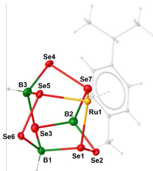
Fig. 3 Molecular structure of 3 . Selected bond lengths ( \text{\AA} ) and angles ( ^\circ ): Ru1-Se1 2.4730(10), Ru1-Se5 2.4767(10), Ru1-Se7 2.4787(11), Se1-Se2 2.3628(12), Se4-Se7 2.3600(12), Se5-Se6 2.3542(12), Se1-B1 2.076(8), Se3-B1 2.065(8), Se6-B1 2.020(8), Se2-B2 2.013(8), Se3-B2 2.065(8), Se7-B2 2.073(8), Se3-B3 2.054(9), Se4-B3 2.014(9), Se5-B3 2.099(8); B2-Se2-Se1 89.6(2), B3-Se4-Se7 90.2(2), B1-Se6-Se5 90.4(2).
