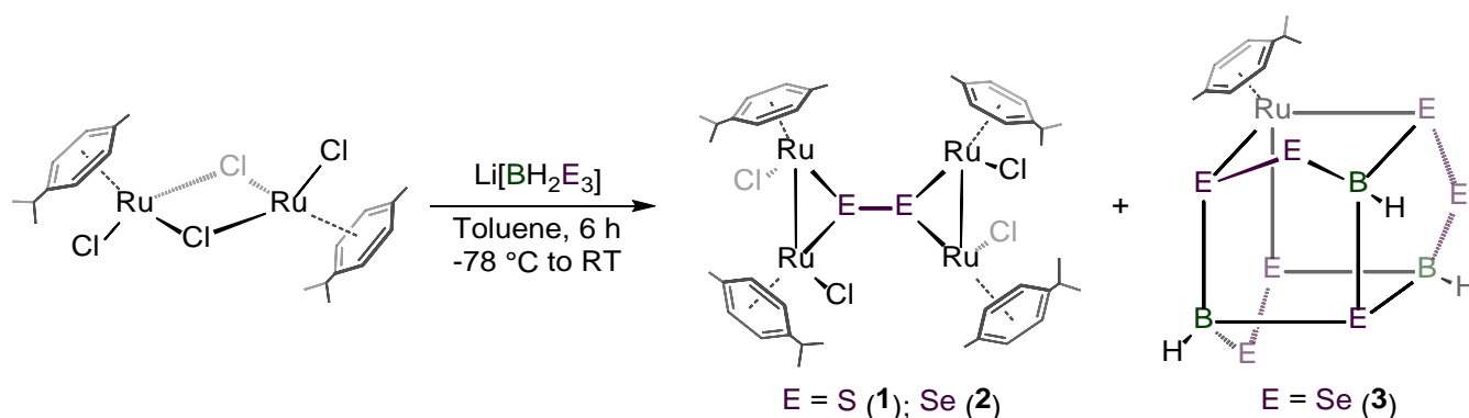
Scheme 1 Synthesis of tetranuclear dichalcogenide complexes of ruthenium.
