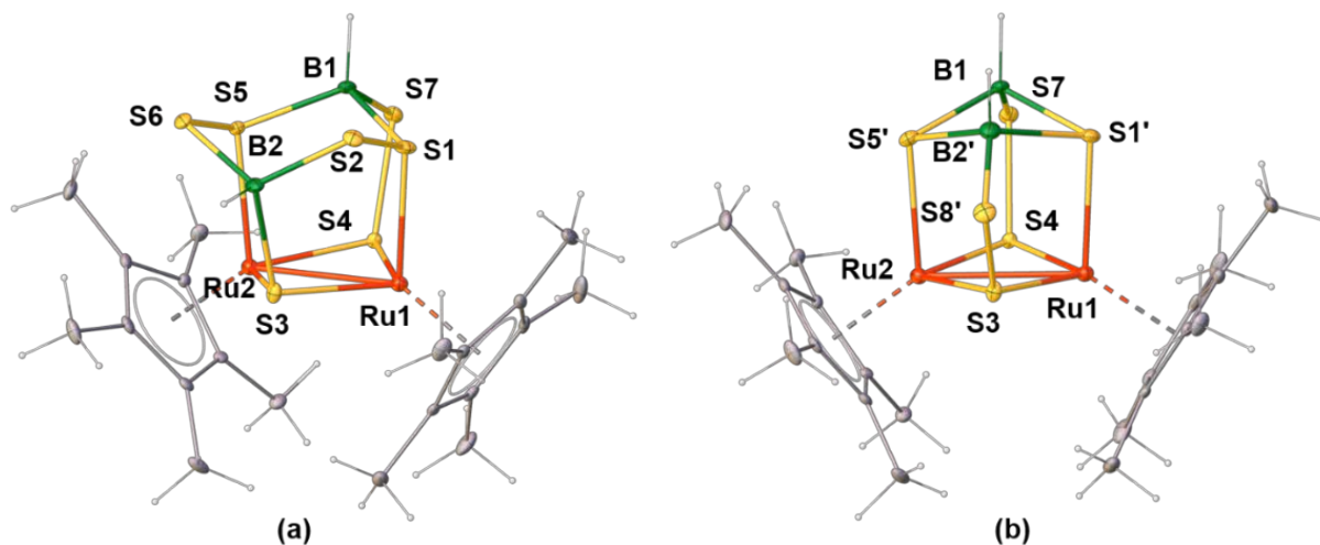
Fig. 4. Molecular structures of (a) 4 and (b) 5 . Selected bond lengths (Å) and bond angles (°). 4 : B1-S1 1.932(5), B1-S5 1.946(11), B1-S7 1.868(6), B2-S2 1.866(13), B2-S3 2.095(12), B2-S6 1.866(14), S1-S2 2.013(2), S5-S6 2.052(14), S4-S7 2.1130(15), Ru1-S1 2.3637(11), Ru1-S3 2.2976(11), Ru1-S4 2.2927(10), Ru2-S3 2.3049(11), Ru2-S4 2.2875(10), Ru2-S5 2.356(12), Ru1-Ru2 2.7804(5), S1-B1-S5 108.8(5), S1-B1-S7 106.6(3), S5-B1-S7 104.8(5). 5 : B1-S1' 1.932(5), B1-S5' 1.91(2), B2'-S1' 2.165(16), B2'-S5' 2.02(3), B2'-S8' 1.816(17), S3-S8' 1.942(5), Ru1-S1' 2.3637(11), Ru2-S5' 2.39(2); S1'-B2'-S5' 92.5(8), S5'-B2'-S8' 114.0(10).
