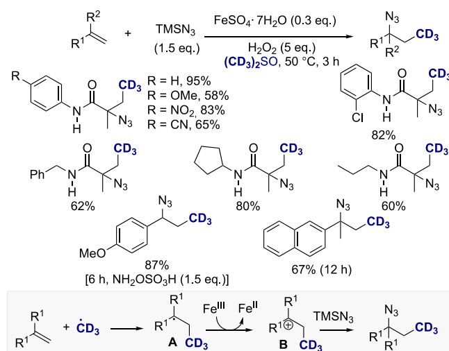
Scheme 41. Azidotrideuteromethylation of acrylamides and styrenes with TMSN 3 / d 6 -DMSO and proposed mechanism
