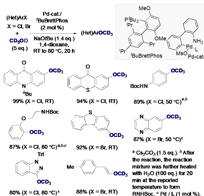
Scheme 72. Pd-catalyzed arylation or vinylation of CD 3 OD
