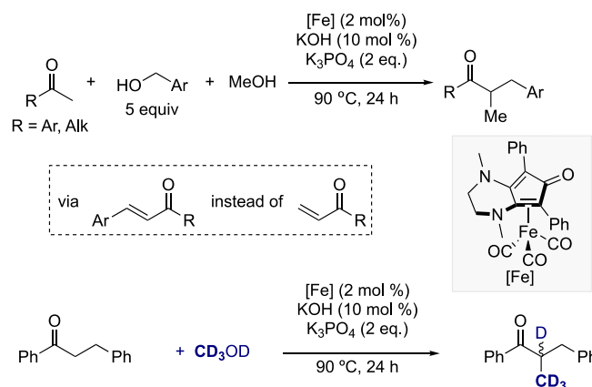
Scheme 23. Tandem three-component alkylation of ketones and mechanistic study
