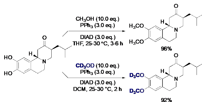
Scheme 66. Synthesis of tetrabenazine and deutertetrabenazine via Mitsunobu reaction with \text{CH}_3\text{OH} or \text{CD}_3\text{OD}
