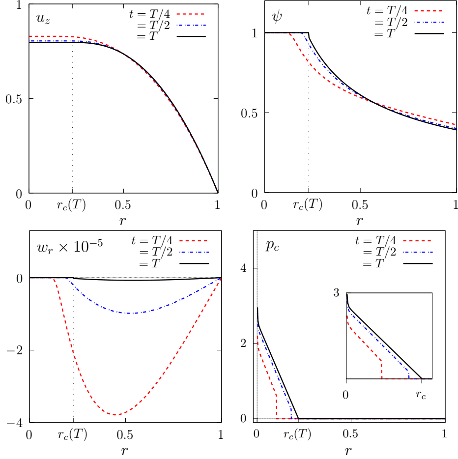
Figure 5: Radial profiles of mixture velocity u_z , reduced volume fraction \psi , migration velocity w_r , and particle contact pressure p_c at different times. Time t = T corresponds to fully-developed flow ( \phi_0 = 0.32 , \phi_m = 0.585 , h = 1/800 ).
