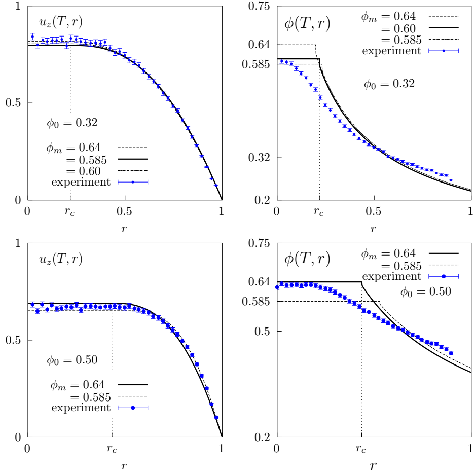
Figure 6: Comparisons of the present migration model with experimental results of Oh et al. [18] for the fully developed flow regime. (top) semi-concentrated case \phi_0 = 0.32 ; (bottom) concentrated case \phi_0 = 0.50 . Note that error bars on the data correspond to experimental uncertainties estimated by Oh et al. [18] based on measurements on the interstitial fluid, and might thus be underestimated for concentrated mixtures.
