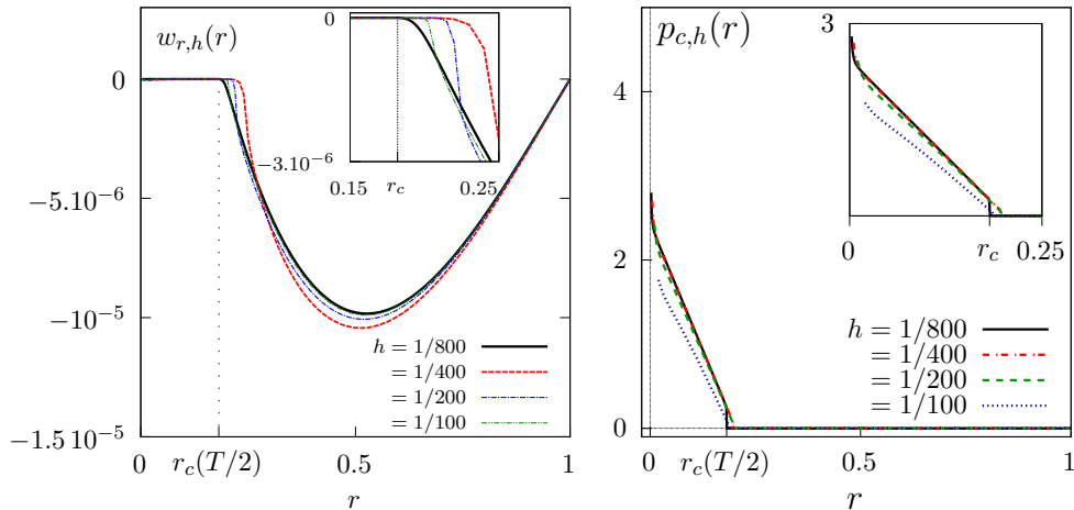
Figure 4: Convergence versus simultaneous time and spatial refinement: Radial profiles at t = T/2 of (left) radial migration velocity w_{r,h}(r) , and (right) particle contact pressure p_{c,h}(r) . Insets show close-ups on the inner plug region.
