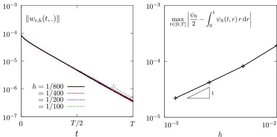
Figure 3: Convergence versus simultaneous time and space mesh refinement. (left) L^2 norm of the radial component w_{r,h} of the particle velocity versus dimensionless time t . (right) Maximum particle mass error versus h .
