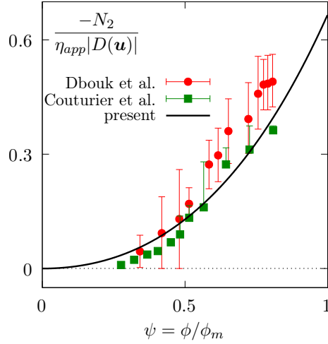
Figure C.7: Steady-state normal stress ratio N_2/\eta_{app}|2D(\mathbf{u})| as a function of reduced volume fraction \psi : comparison between the predictions the rheological model (with values indicated in table 2) and experimental data of Dbouk et al. [58] and Couturier et al. [59].
