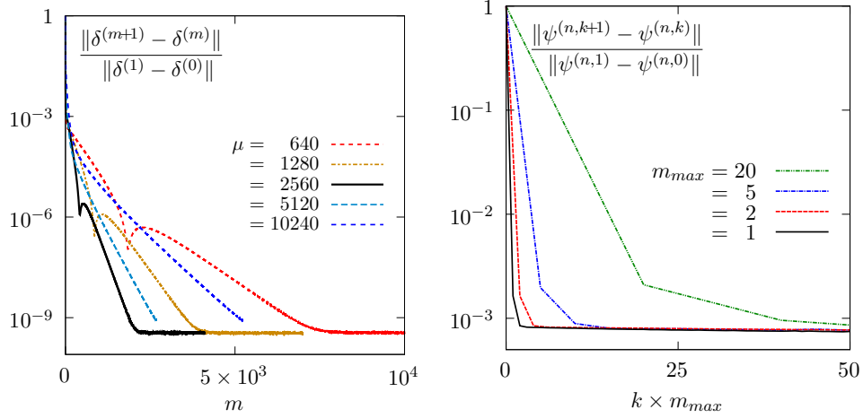
Figure 2: Convergence of the two inner loops at t = T/4 ( h = 1/400 ). (left) Convergence of the augmented Lagrangian loop: normalised relative error on the auxiliary variable \delta^{(m)} versus iteration number m for various values of augmentation parameter \mu . (right) Convergence of the fixed point loop: relative error for the volume fraction \psi^{(n,k)} versus total iteration number k \times m_{max} for various values of m_{max} .
