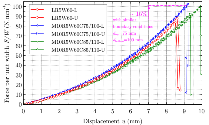
Figure 7: Load per unit width F/W versus displacement u curves for LR5W60, M10R5W60C75/100 and M10R5W60C85/110 configurations
