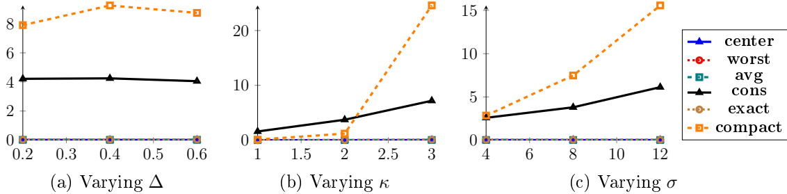
Figure 9: STP: Average solution times in seconds on instances format ( \kappa ) for each algorithm when varying one of the parameters.
