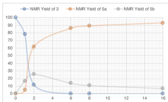
Figure 3. Kinetic profile of Pd-catalyzed C–H bond arylation of complex 3 with 4-bromobenzotrifluoride. ^{19}\text{F} NMR yield using fluorobenzene as internal standard.
