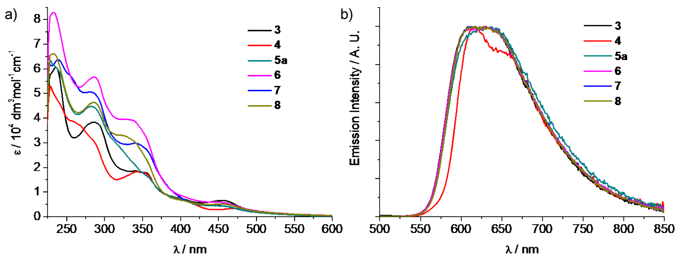
Figure 5. (a) Absorption and (b) normalized emission spectra of complexes 3–8 in deoxygenated \text{CH}_2\text{Cl}_2 ( \lambda_{\text{ex}} = 365 nm, concentration \sim 1 \times 10^{-5} M) at 298 K.
