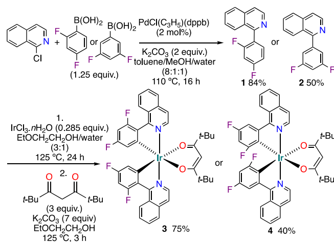
Scheme 1. Preparation of bis[2-(3,5-difluorophenyl)isoquinolinyl](2,2,6,6-tetramethyl-3,5-heptanedionato)-Ir(III) ( 3 ) and bis[2-(4,6-difluorophenyl)isoquinolinyl](2,2,6,6-tetramethyl-3,5-heptanedionato)-Ir(III) ( 4 ).
