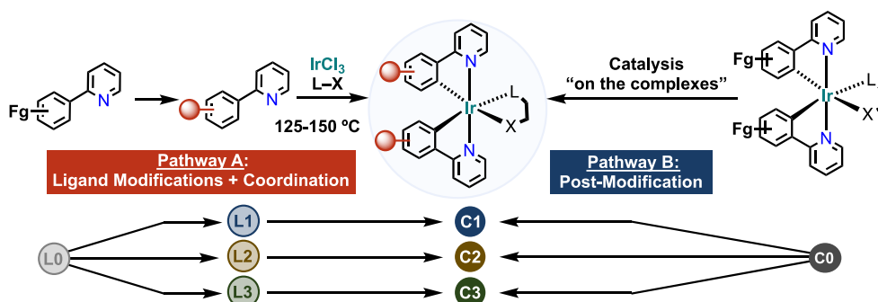
Figure 1. Different approaches to prepare functionalized Ir(III) complexes
