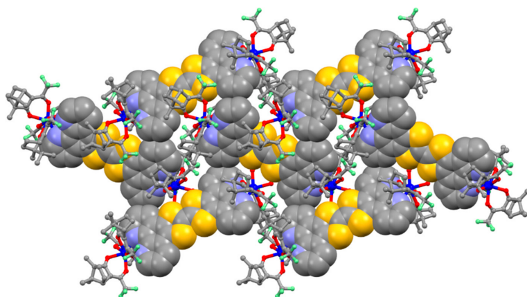
Figure 3. Crystal packing of (2)·2(C 6 H 14 ) with the triads L and Dy( facam ) 3 units drawn respectively in spacefill and ball and sticks representation.
