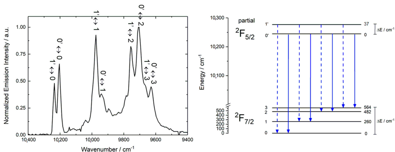
Figure 4. (Left) Solid-state emission spectrum of 1 recorded at 10 K under excitation of 22,220\text{ cm}^{-1} (450 nm) with the proposed transitions between the crystal field sublevels of the ^2\text{F}_{5/2} \rightarrow ^2\text{F}_{7/2} emission band. (Right) Energy diagram of the ^2\text{F}_{5/2} excited state and ^2\text{F}_{7/2} ground state obtained from the solid-state emission spectrum measured at 10 K.
