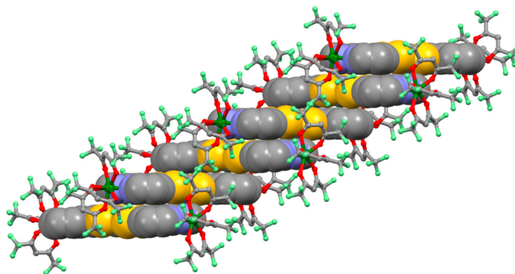
Figure 2. Crystal packing of (1)·2(C 7 H 16 ) highlighting the 1D stacking of L (spacefill representation). The Yb(hfac) 3 units are represented by balls and sticks.
