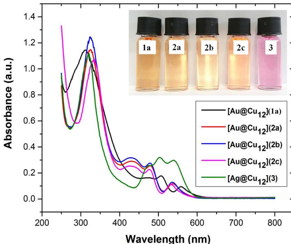
Figure 2. UV-vis absorption spectra of salts of 1a + , 2a + , 2b + , 2c + , and 3 + in CH 2 Cl 2 . The inset shows photographs in CH 2 Cl 2 at ambient temperature.
