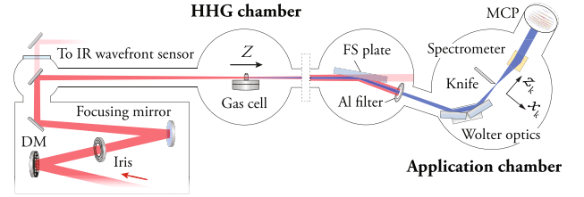
FIGURE 1: Schematic representation of the experimental setup. The spatially filtered IR beam (red) is first wavefront-corrected by a deformable mirror before it goes through an iris and is reflected by a focusing mirror. High-order harmonics (blue) are generated in an argon gas cell. The IR is filtered out by an IR antireflection-coated fused silica plate followed by an aluminum filter. In the application chamber, the harmonic beam is focused by the Wolter optics. The knife is placed around the focus, and the beam is detected by a flat-field spectrometer.
