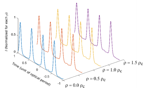
Fig. 9. The intensity temporal profiles for jet position 15 mm before IR focus at radii specified by white lines in Fig. 7. We compare the case with (b) and without (a) the pinhole but at different radii for which harmonic intensities are comparable. The values of \rho are chosen around the critical radius, defining the radius at which the energy is equally shared between the inner and outer region. \rho_c = 50 \mu\text{m} for the apertured case and \rho_c = 167 \mu\text{m} for the free case. In figs. (c) and (d), the distributions have been normalized for each value of \rho .
