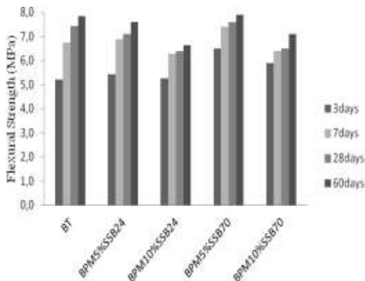
Figure 7. Evolution of the flexural strength of different types of concrete
