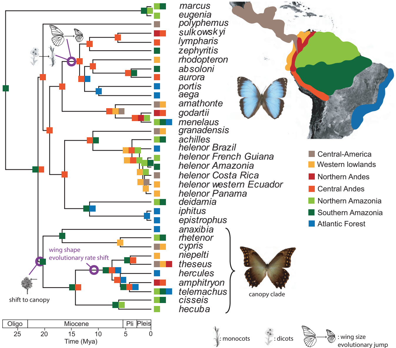
FIGURE 4 Historical biogeography inferred for the genus Morpho . The most likely states are indicated at the nodes. The different clade-specific ecological factors are also indicated on the tree. The two pictures of Morpho depict the typical wing shapes associated with each microhabitat—top: short rounded wings characteristic of the understory species, bottom: elongated wings towards the apex characteristic of the canopy clade
