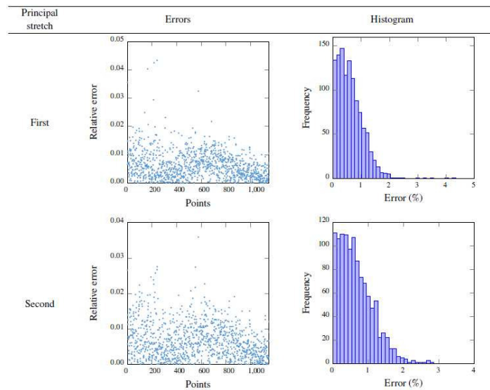
Fig. 13 Yeoh model: final results
