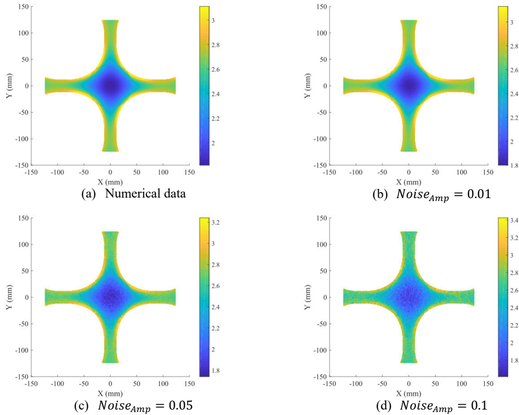
Fig. 2 Maximal principal stretch fields for a displacement equal to 70 mm: numerical and noised data
