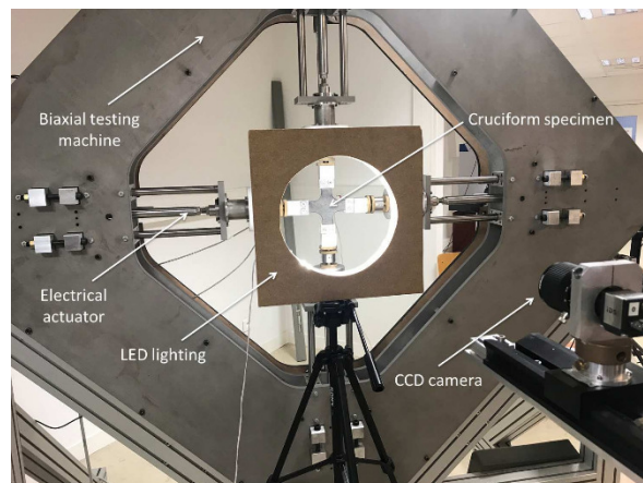
Fig. 5 Experimental setup
