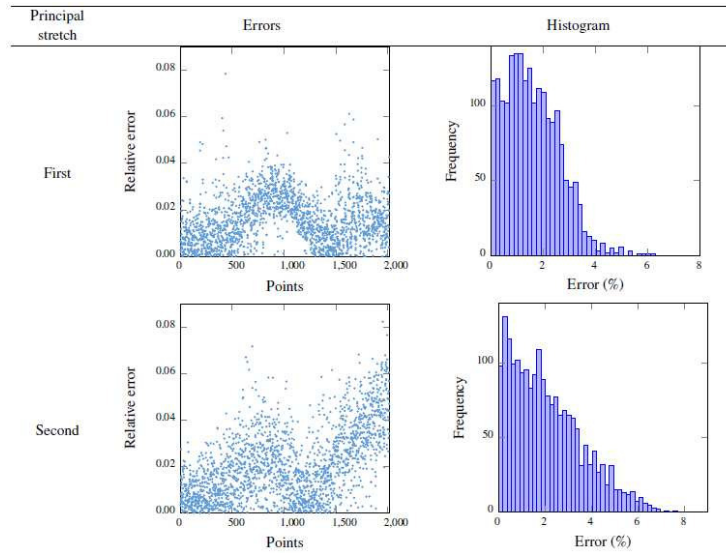
Fig. 12 Mooney model: final results
