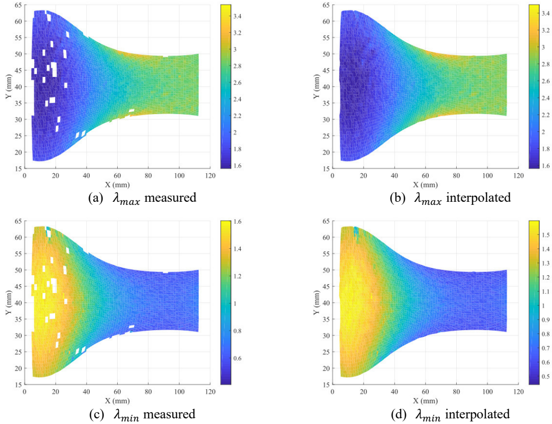
Fig. 10 Principal stretch fields for a displacement equal to 70 mm
