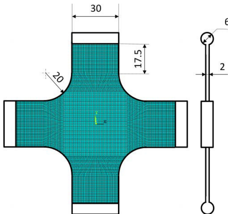
Fig. 1 Specimen geometry (dimensions in mm) and FE mesh. It should be noted that with FEMU, a problem is often encountered, which is to determine the correct force distribution along the boundary of the specimen. Indeed, slippage in the grips inducing heterogeneities in the force distribution cannot be really measured. The problem is resolved by adding small cylinders at the end of the four branches of the specimen and by using suitable grips. They prevent slipping into the machine's grips
