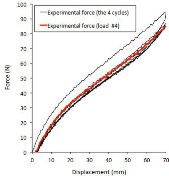
Figure 7: Mechanical response in terms of the horizontal force versus the displacement applied
