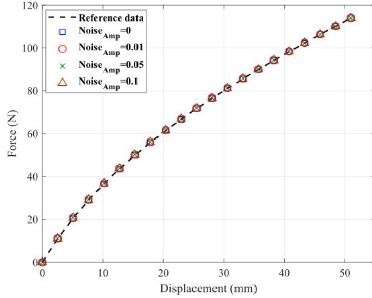
Fig 3 Force response versus displacement for parameters of Table 3 (Mooney model)
