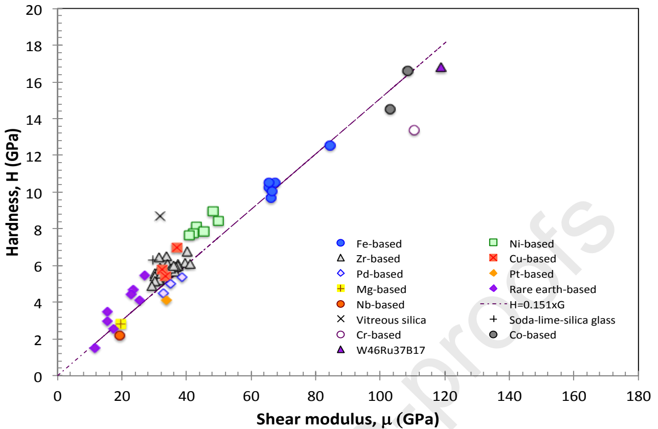
Fig. 12. Hardness, H , plotted as a function of the shear modulus, \mu , illustrating the influence of the chemical system.
