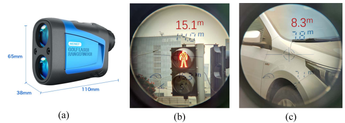
Fig. 11. The laser rangefinder and its use cases. The distances labeled in red are the results measured by our system and the distances marked in dark blue are that measured by the rangefinder which represent the ground truth. (a) The laser rangefinder; (b) The measurement case of PTL; (c) The measurement case of vehicle.
