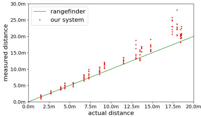
Fig. 12. The results measured by the rangefinder and the proposed system. x-axis: the actual distance; y-axis: the measured distance.
