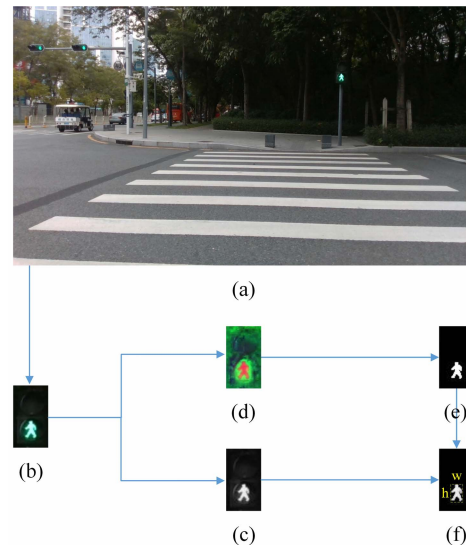
Fig. 7. Diagram of pedestrian traffic light recognition: (a) RGB image; (b) candidate; (c) gray image; (d) HSV image; (e) traffic light mask; (f) the shape of traffic light.
