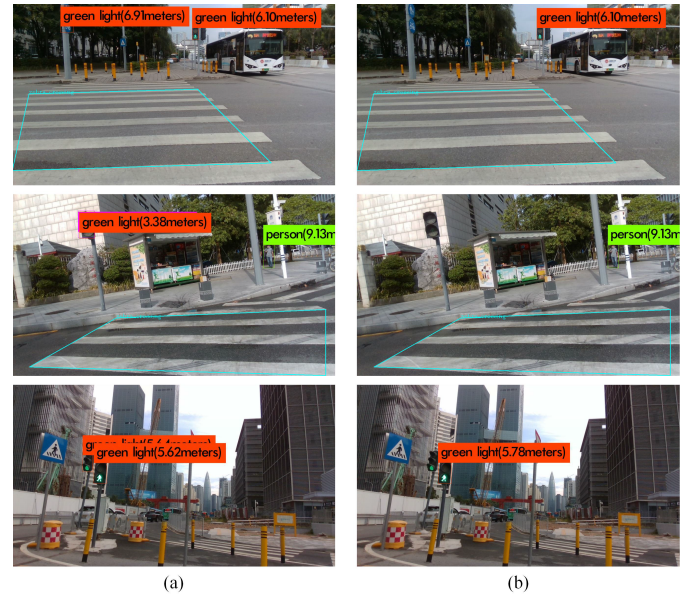
Fig. 10. The detected results by YOLOv4 (a) and our method (b).
