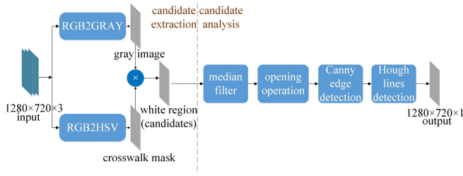
Fig. 4. The framework of crosswalk detector.
