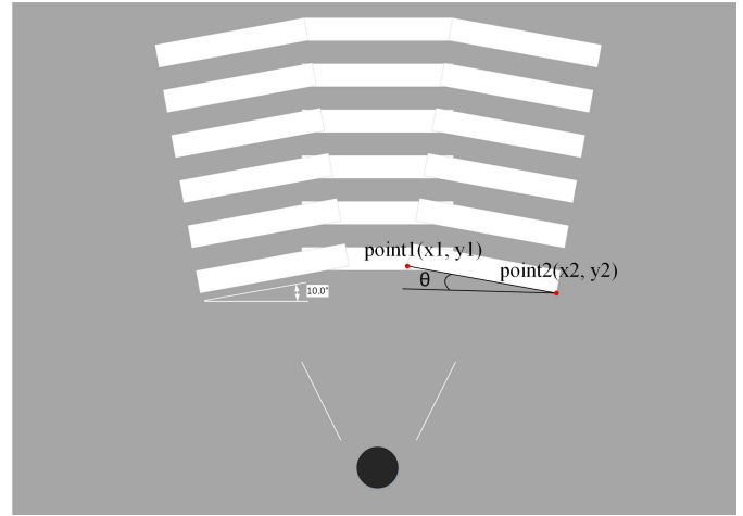
Fig. 6. The sketch of \theta , which ranges in [0, 10^\circ] .
