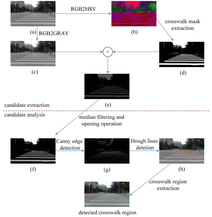
Fig. 5. Diagram of candidate extraction and candidate analysis: (a) input image; (b) HSV image; (c) gray image; (d) crosswalk mask; (e) white region(candidates); (f) result of median filter; (g) result of Canny edge detection; (h) result of Hough transform.
