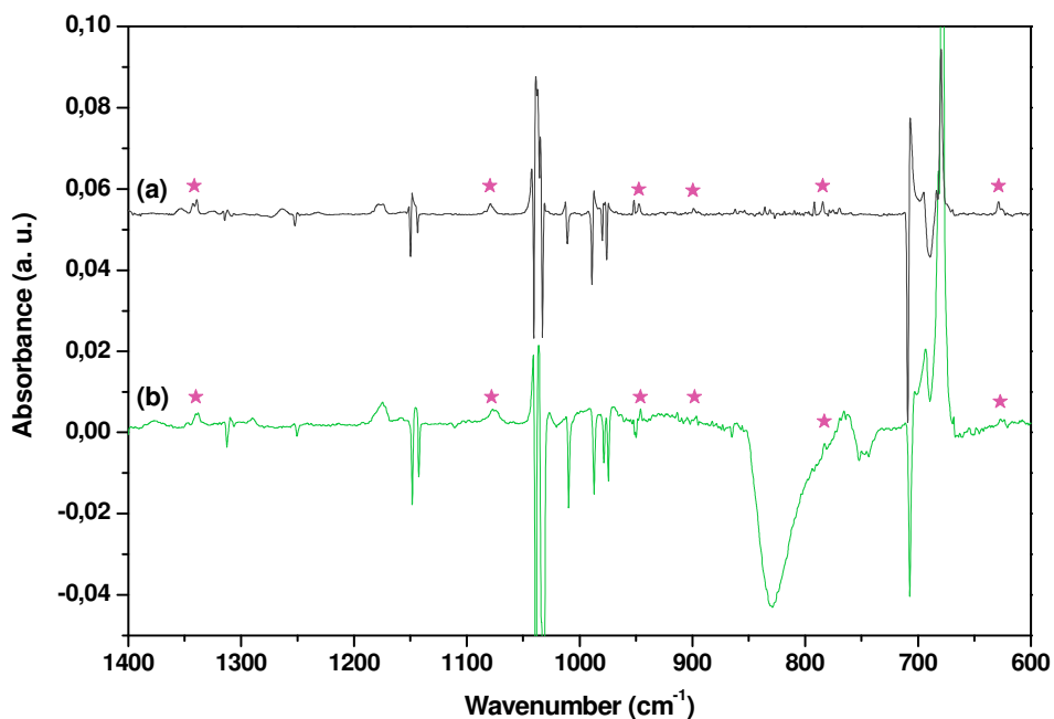
296 Figure 4 – Comparison of the FTIR difference spectrum after-before irradiation (with the 297 mercury lamp, 70 K) of a pure benzene ice (a) and a C_6H_6:HCN 4:1 ice (b) on which the 298 absorption bands assigned to fulvene are identified by stars 299
