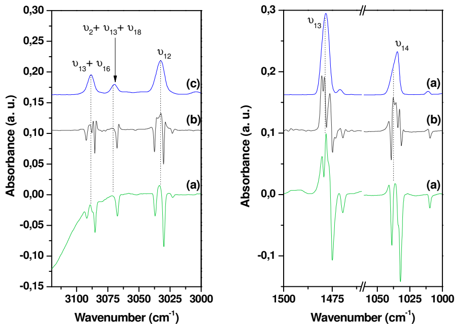
291 Figure 3 – Comparison of the FTIR difference spectrum after-before irradiation (with the 292 mercury lamp, 70 K) of a co-condensed ice C_6H_6:HCN 4:1 (a) and a pure benzene ice (b) with 293 the FTIR spectrum of a an amorphous benzene ice (50 K, c) 294
