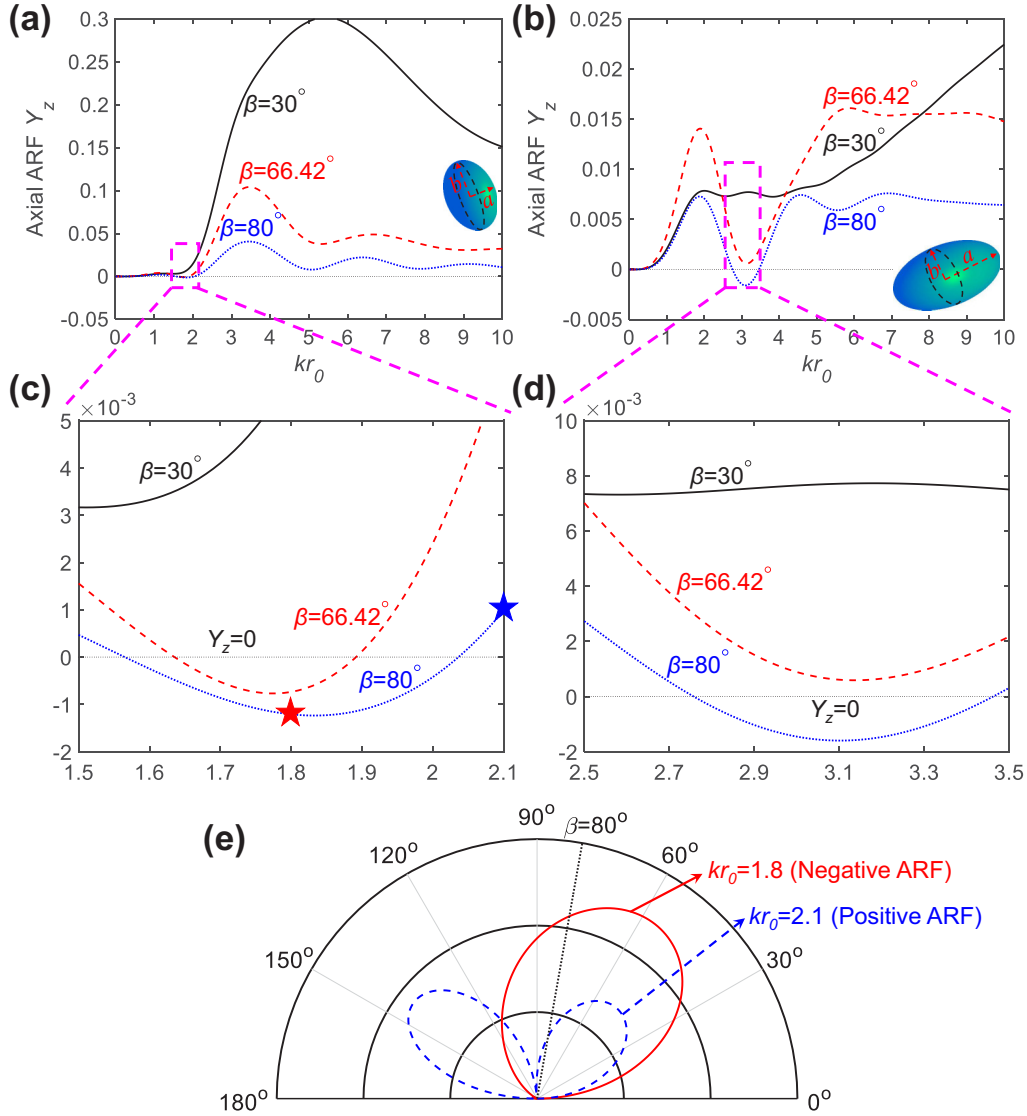
FIG. 4. (a) The axial ARF of the rigid oblate spheroid with aspect ratio a/b = 1/2 with r_0 = b ( a < b ). The order of the Bessel beam is M = 1 with cone angles \beta = 30^\circ, 66.42^\circ , and 80^\circ . (b) Like panel (a) except that the particle is the prolate spheroid with a/b = 2 and r_0 = a ( a > b ). Panels (c) and (d) depict the enlarged view of the negative ARF region for the rigid oblate and prolate spheroids, respectively. (e) Angular dependence of the scattered form functions vs the scattered polar angle \theta_s for the oblate spheroid in the first-order HBB with \beta = 80^\circ for kr_0 = 1.8 [red solid line, corresponding to the red solid pentagram in (c)] and kr_0 = 2.1 [blue dash line, corresponding to the blue solid pentagram in (c)]. The black dotted line denotes the direction of the incident wave vector with \theta_s = \beta . Negative axial ARFs exist when the scattering in the forward hemisphere is relatively stronger than that in the backward hemisphere.
