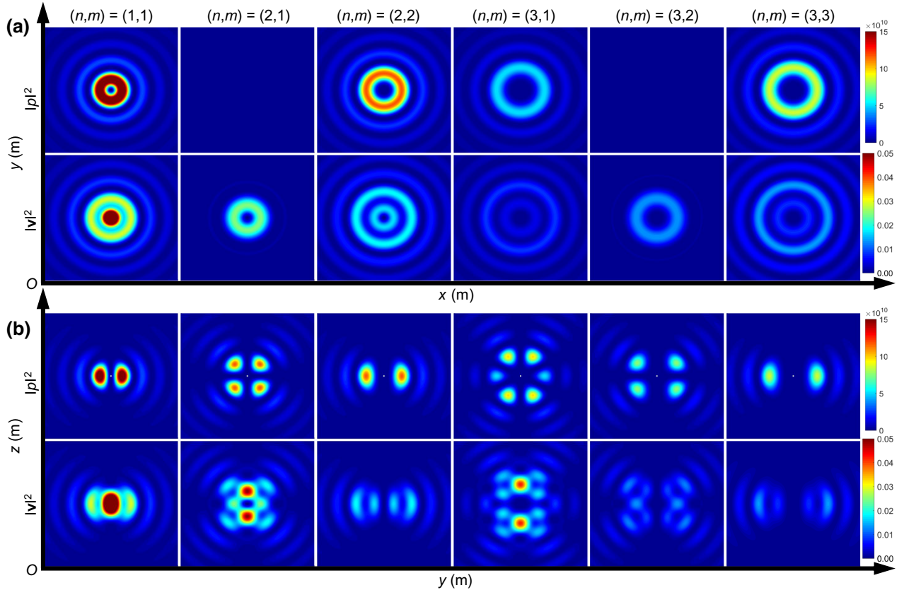
FIG. 2. Square of the pressure modulus |p|^2 and square of the velocity modulus |\mathbf{v}|^2 in (a) the (x, y) plane and (b) the (y, z) plane for a single SBV with different orders (n, m) and the same input power [corresponding to an amplitude A_0 = 10^6 for (n, m) = (1, 1) and normalized according to Eq. (2) for other orders].
