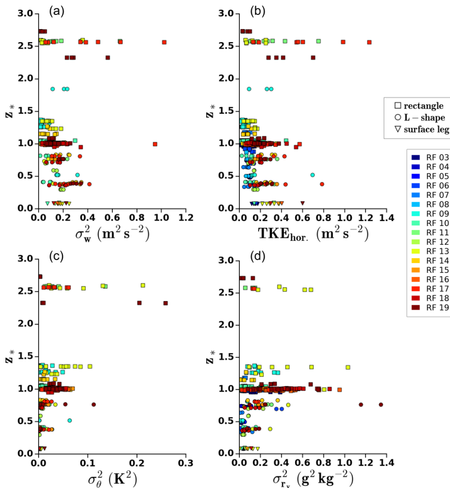
Figure 15. Normalized vertical profiles of the variance of (a) vertical velocity, (b) horizontal turbulent kinetic energy, (c) temperature and (d) water vapor mixing ratio. Flight numbers are indicated in the top right box. For the water vapor mixing ratio, only the legs with a green or a yellow combined flag have been considered. The normalized altitude z_* is defined by z/LCL with LCL, the lifting condensation level.
