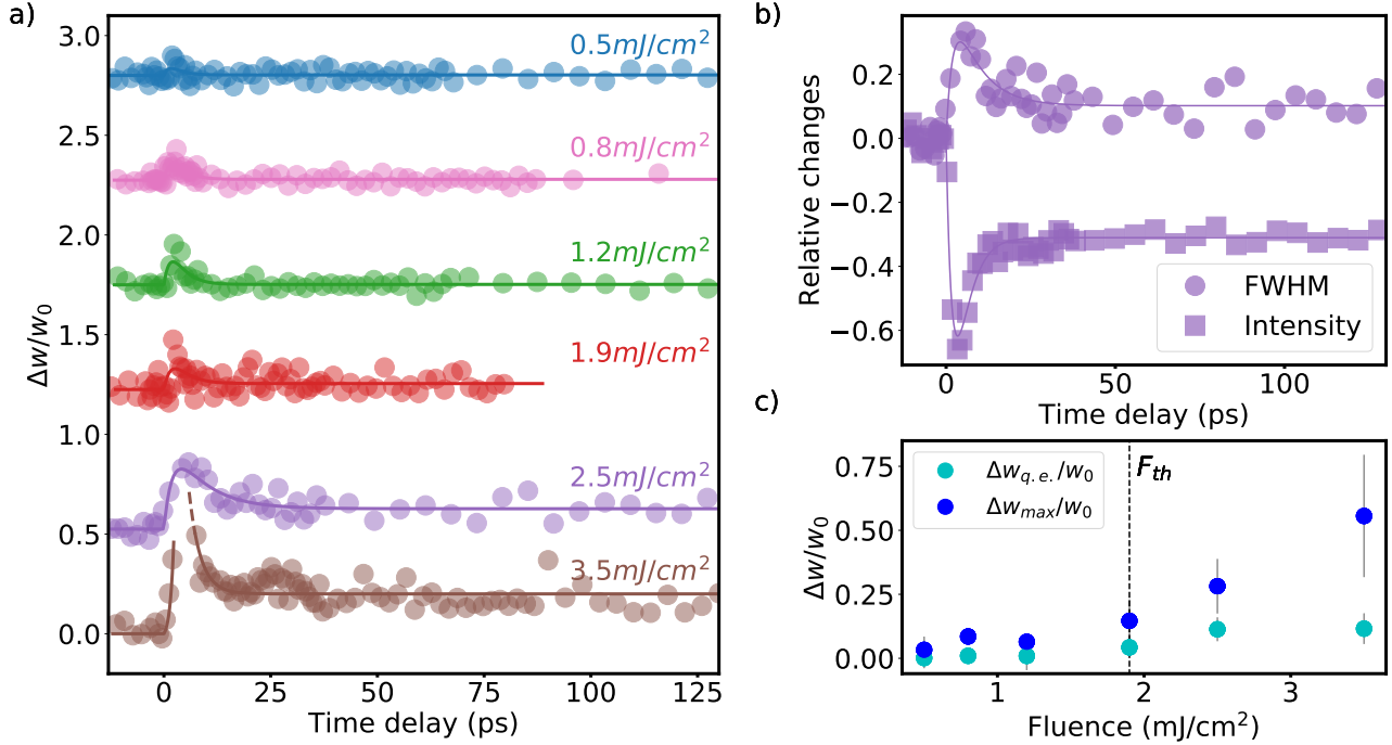
FIG. 9. a) Temporal evolution of \Delta w/w_0 , the relative change of the peak FWHM for different incident fluences. The curves are vertically shifted for clarity. b) Relative intensity (squares) and FWHM (circles) temporal changes at an incident fluence of 2.5 mJ/cm 2 , c) Relative changes of the FWHM maximum \Delta w_{max}/w_0 (averaged over the four points around the maximum) and after the time recovery at quasi-equilibrium \Delta w_{q.e.}/w_0 (averaged over the last twenty points of each curve in a)) where w_0 is the initial satellite width. Error bars represent the standard deviation derived from the average.
