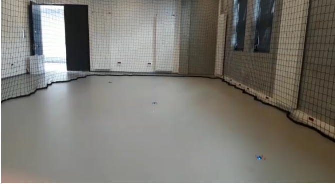
Fig. 1. Experiment with three Crazyflie drones in the flight arena.
