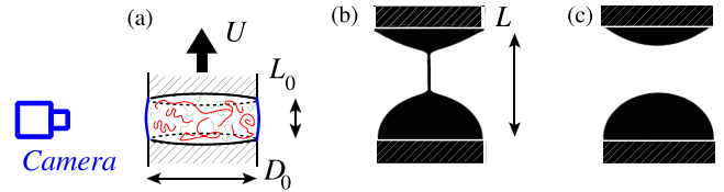
Figure 1. (a) Liquid capillary bridge of the polymer solution sandwiched between parallel disks of diameter D_0 and initial height L_0 before being stretched with a velocity, U . (b) The top disk reaches the final stretching height, L , and a thinning filament is observed. (c) Breakup of the liquid bridge.
