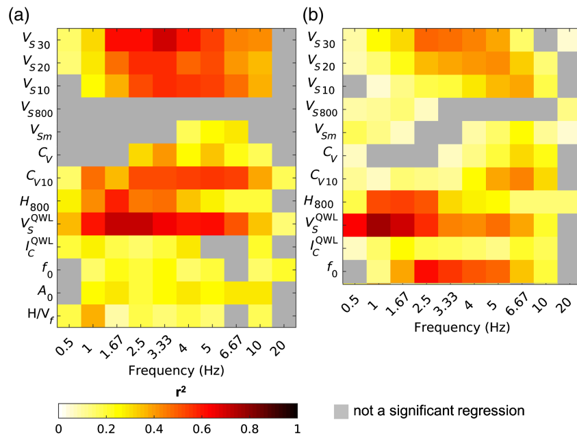
Figure 1 (reproduced from Bergamo et al., 2020). Quality of the regressions obtained between (frequency-dependent) Fourier amplification factors and each individual proxy. Note that the values of V_S^{QWL} , I_C^{QWL} and H/V_f change with frequency. The color code corresponds to the value of the coefficient of determination R^2 . Panel (a) refers Swiss data and panel (b) to Japanese data.
