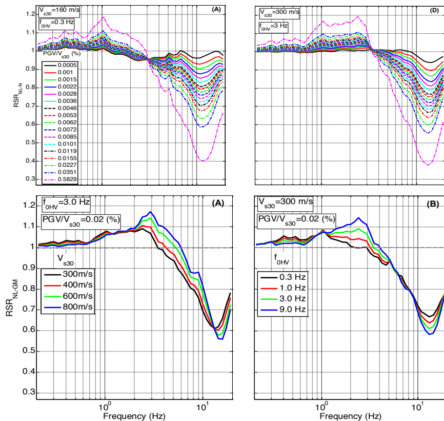
Figure 5 (reproduced from Derras et al., 2020): Variation of RSR_{NL-L}(f; PGV/V_{S30}; V_{S30}, f_{0HV}) predicted for increasing values of PGV/V_{S30} and fixed values of V_{S30} and f_{0HV} (top row), or for fixed strain and f_{0HV} values and different V_{S30} values (300, 400, 600, 800 m/s, bottom left), or for fixed strain and V_{S30} values and different f_{0HV} values (0.3, 1.0, 3.0, 9.0 Hz, bottom right). The values of PGV/V_{S30} (in %), V_{S30} and f_{0HV} are provided in each frame,.
