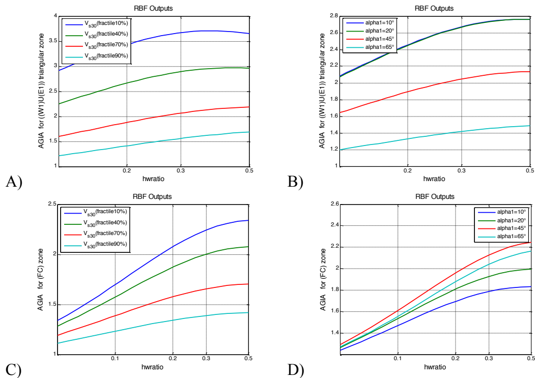
Figure 10: Example predictions for the Arias Intensity, for the W1UE1 zone in triangular valleys (cases A and B on top), and for the central fault part FC of trapezoidal valleys (cases C and D on bottom). The different cases considered are listed in Table 4
