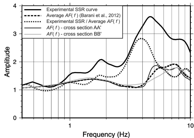
Figure 7 (reproduced from Barani et al 2014): Comparison between the numerical amplification functions AF(f) for two cross-sections (AA' and BB') and the experimental AF(f) obtained by Massa et al. (2010) at the Narni ridge (central Italy).
