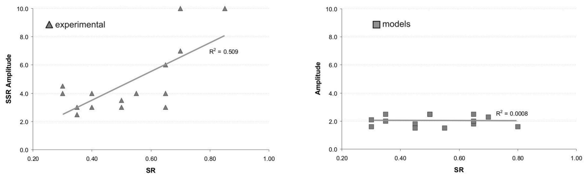
Figure 6 (reproduced from Massa et al (2014): Relationships between topographic shape ratio h/w and SSR (Standard Spectral Ratio) amplitude as obtained from experimental (left-hand panel) and numerical (right-hand panel) data.. (Data collected from published, noteworthy studies, grey triangles correspond to instrumental observations (left-hand side), grey squares to numerical simulation (right-hand side, grey lines to simple regressions).
