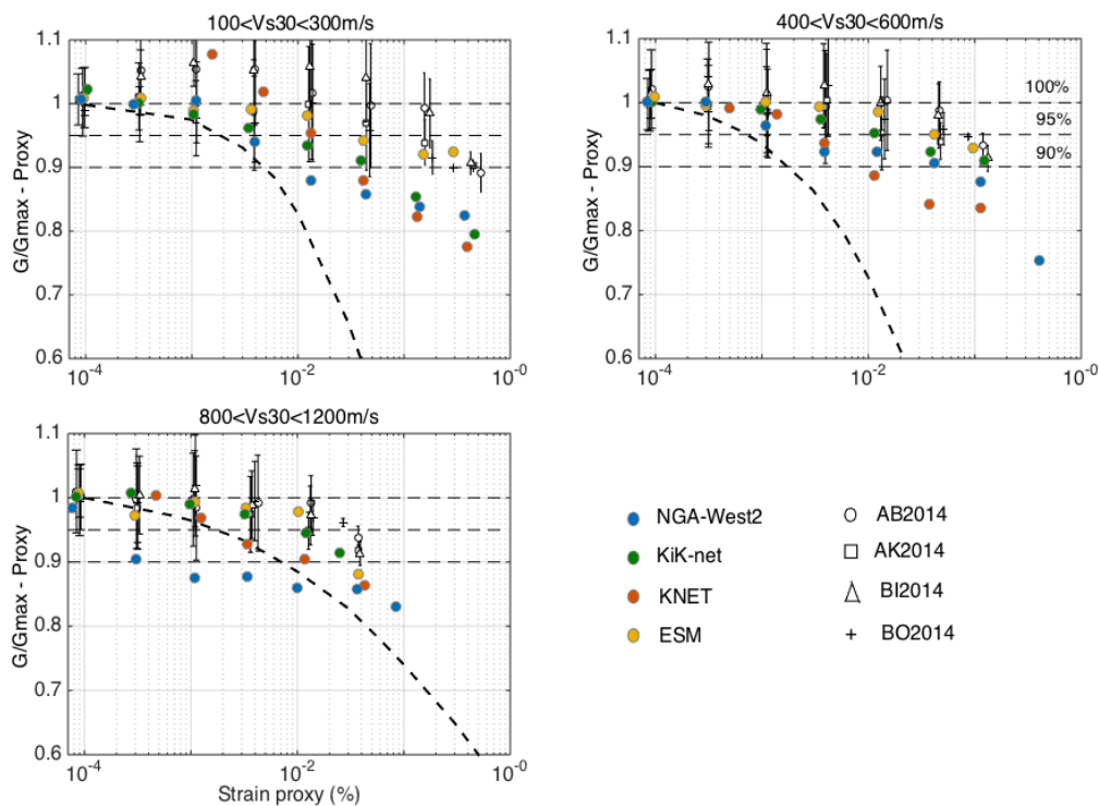
Figure 4 (reproduced from Guéguen et al., 2019): Comparison of predicted and observed nonlinearities in terms of the shear modulus reduction G/G_{max} (estimated from PGA to strain proxy ratios in different strain intervals) as a function of the strain proxy ( PGV/V_{S30} ). Open symbols correspond to estimates according to four GMPEs (AB2014: Abrahamson et al., 2014; AK2014: Akkar et al., 2014b; BI2014: Bindi et al., 2014; BO2014: Boore et al., 2014). Filled, colored circles correspond to average values from the four databases for three site classes, for strain proxies larger than 10^{-4} %. Thin horizontal dashed lines correspond to 100%, 95% and 90% of the G/G_{max} values. Bold dashed lines for each V_{S30} class, are standard G-\gamma curves for clay ( PI=15\% ), sand and rock-like soil from Zhao et al. (2015), respectively.
