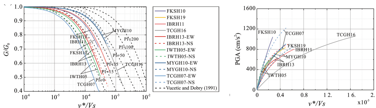
Figure 3 (reproduced from Wang et al., 2019): Instrumentally derived relationships between shear strain and shear modulus ratio (left), compared with laboratory G-\gamma measurements by Vucetic and Dobry (1991), and between shear strain proxy and peak ground acceleration (right).
