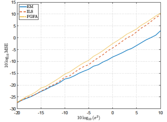
Fig. 6. MSEs of \hat{\theta} = (\hat{r}, \hat{c}^T)^T for FGFA, ILS and EM (proposed method) versus noise power \sigma^2 (500 Monte Carlo runs) for a von Mises-Fisher prior ( \mu = [\sin(\pi/4)\cos(\pi/3), \sin(\pi/4)\sin(\pi/3), \cos(\pi/4)]^T and \kappa = 2 ).
