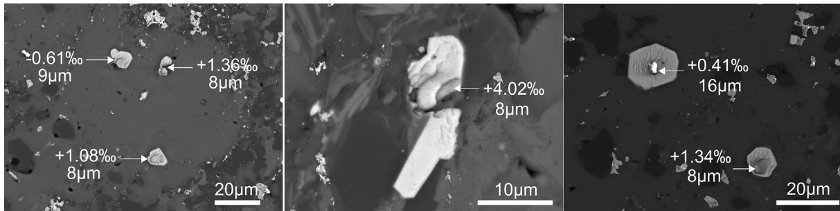
Fig. 6. SEM pictures of micropyrrites in GIS68.9. (a) and (b) Fe isotopic compositions measured in pyrites of 8 to 9 \mu\text{m} size. This size category shows an isotopic range up to 4‰, showing the absence of correlation between \delta^{56}\text{Fe} and the size of the pyrite; c) Fe isotopic compositions of two hexagonal pyrites of 16 \mu\text{m} and 8 \mu\text{m} in size. These pyrites recorded an isotopic difference of 1‰, located at 30 \mu\text{m} from each other, meaning that iron isotopic compositions are not controlled by the shape of the pyrite.
